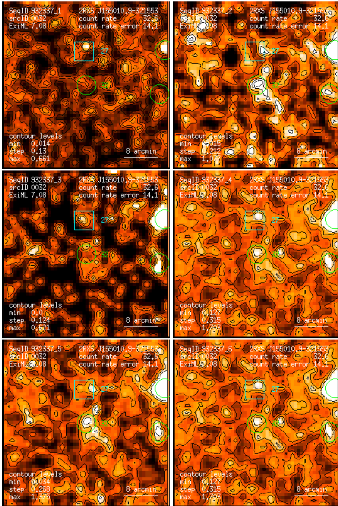
Figure 32: RASS 932337: detection 0032: band rate images, Gaussian filter: (1) PSPC channels 11 – 41, (2) 52 – 90, (3) 91 – 201, (4) 11 – 235, (5) 52 – 201, (6) 11 – 201. Broad band rates in counts/ks. Band rate contour levels in counts/ks/arcmin 2 .
