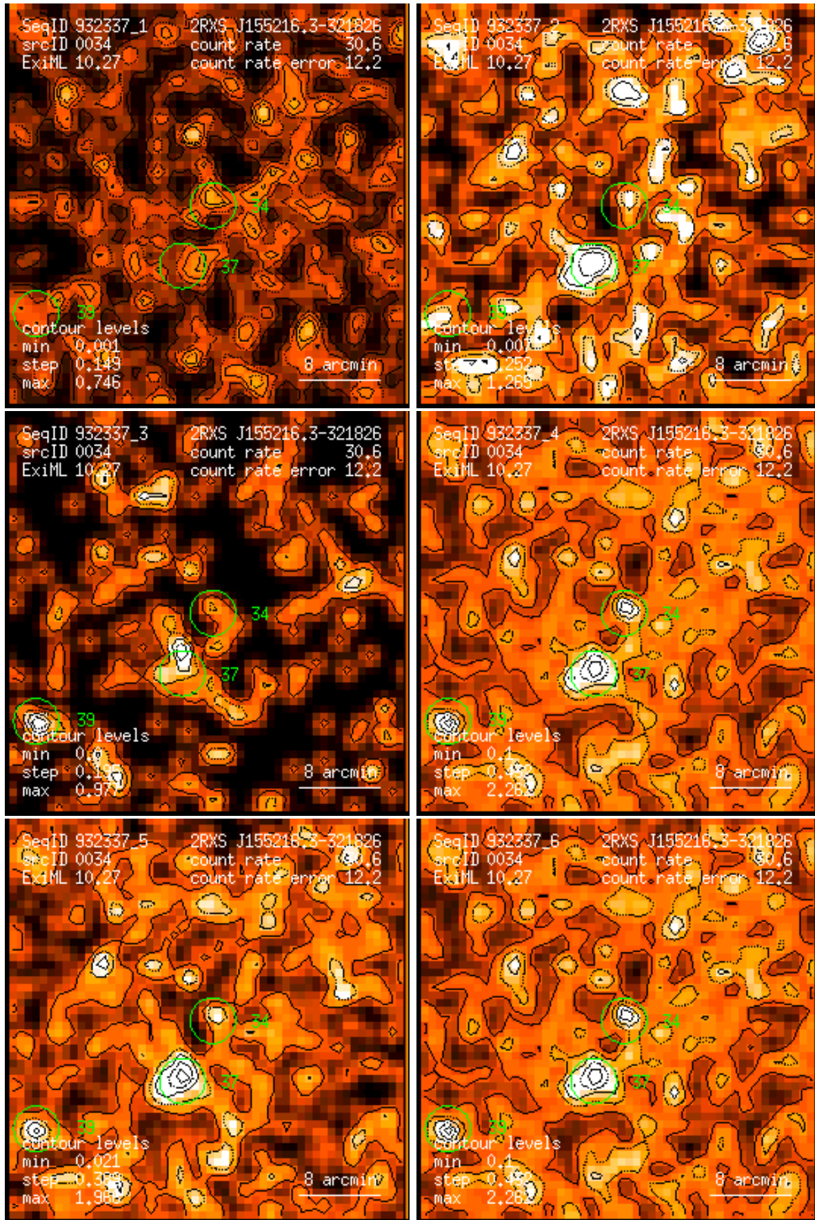
Figure 34: RASS 932337: detection 0034: band rate images, Gaussian filter: (1) PSPC channels 11 – 41, (2) 52 – 90, (3) 91 – 201, (4) 11 – 235, (5) 52 – 201, (6) 11 – 201. Broad band rates in counts/ks. Band rate contour levels in counts/ks/arcmin 2 .
