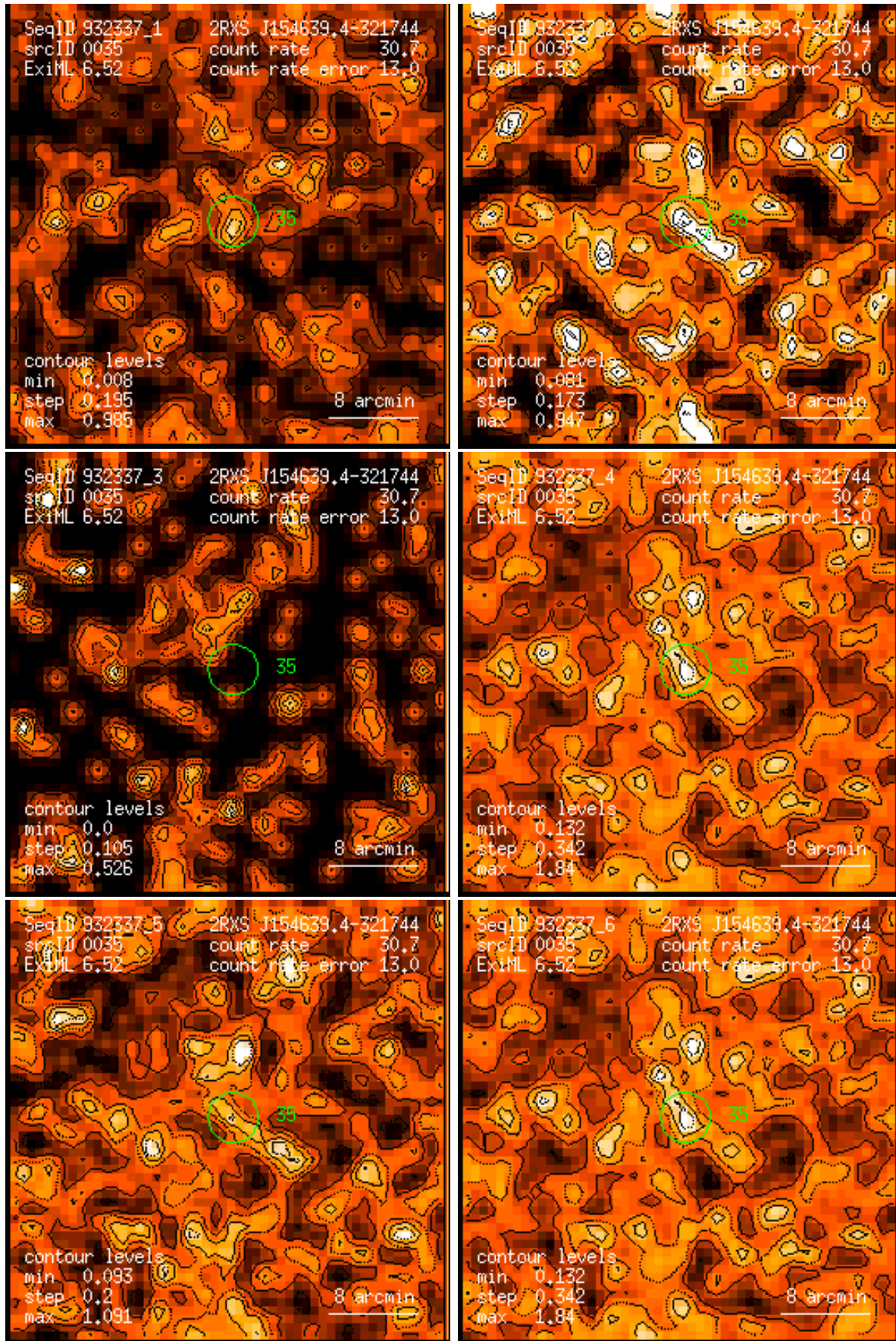
Figure 35: RASS 932337: detection 0035: band rate images, Gaussian filter: (1) PSPC channels 11 – 41, (2) 52 – 90, (3) 91 – 201, (4) 11 – 235, (5) 52 – 201, (6) 11 – 201. Broad band rates in counts/ks. Band rate contour levels in counts/ks/arcmin 2 .
