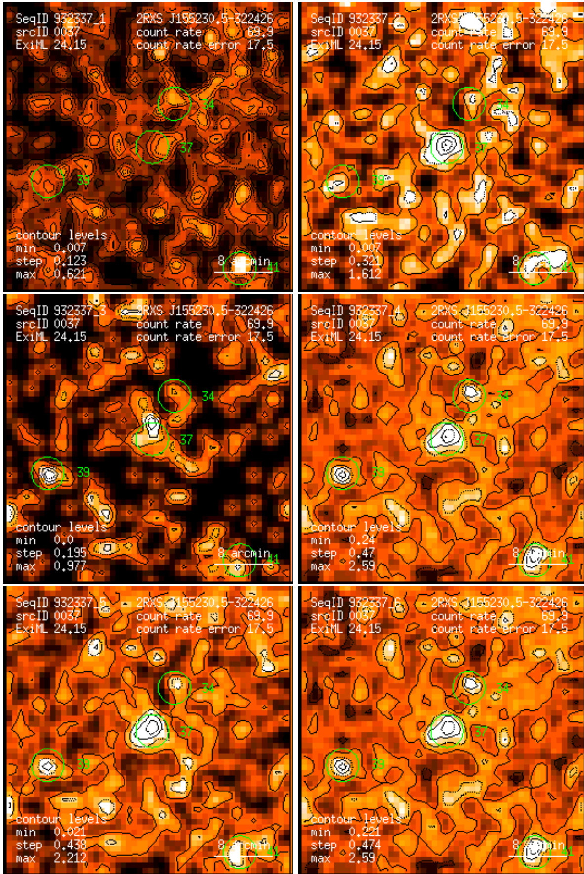
Figure 37: RASS 932337: detection 0037: band rate images, Gaussian filter: (1) PSPC channels 11 – 41, (2) 52 – 90, (3) 91 – 201, (4) 11 – 235, (5) 52 – 201, (6) 11 – 201. Broad band rates in counts/ks. Band rate contour levels in counts/ks/arcmin 2 .
