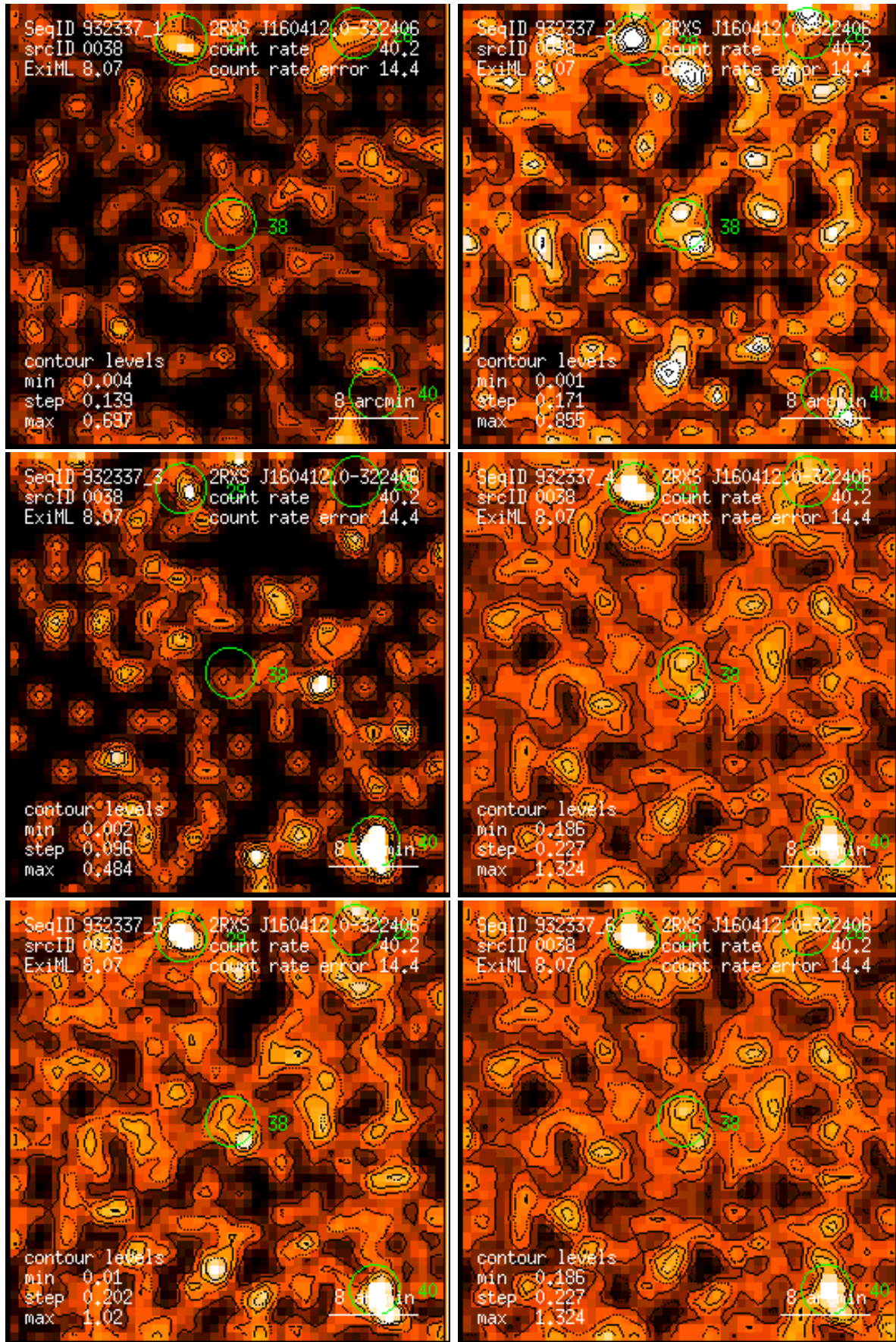
Figure 38: RASS 932337: detection 0038: band rate images, Gaussian filter: (1) PSPC channels 11 – 41, (2) 52 – 90, (3) 91 – 201, (4) 11 – 235, (5) 52 – 201, (6) 11 – 201. Broad band rates in counts/ks. Band rate contour levels in counts/ks/arcmin 2 .
