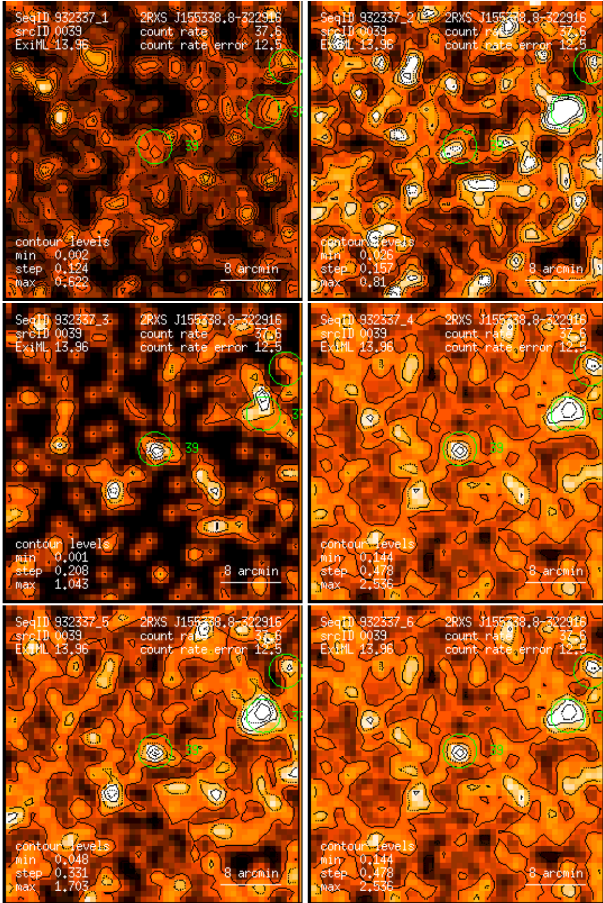
Figure 39: RASS 932337: detection 0039: band rate images, Gaussian filter: (1) PSPC channels 11 – 41, (2) 52 – 90, (3) 91 – 201, (4) 11 – 235, (5) 52 – 201, (6) 11 – 201. Broad band rates in counts/ks. Band rate contour levels in counts/ks/arcmin 2 .
