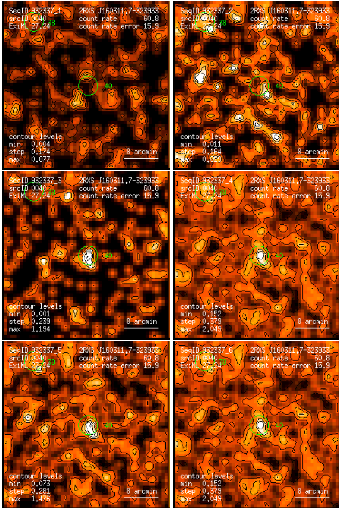
Figure 40: RASS 932337: detection 0040: band rate images, Gaussian filter: (1) PSPC channels 11 – 41, (2) 52 – 90, (3) 91 – 201, (4) 11 – 235, (5) 52 – 201, (6) 11 – 201. Broad band rates in counts/ks. Band rate contour levels in counts/ks/arcmin 2 .
