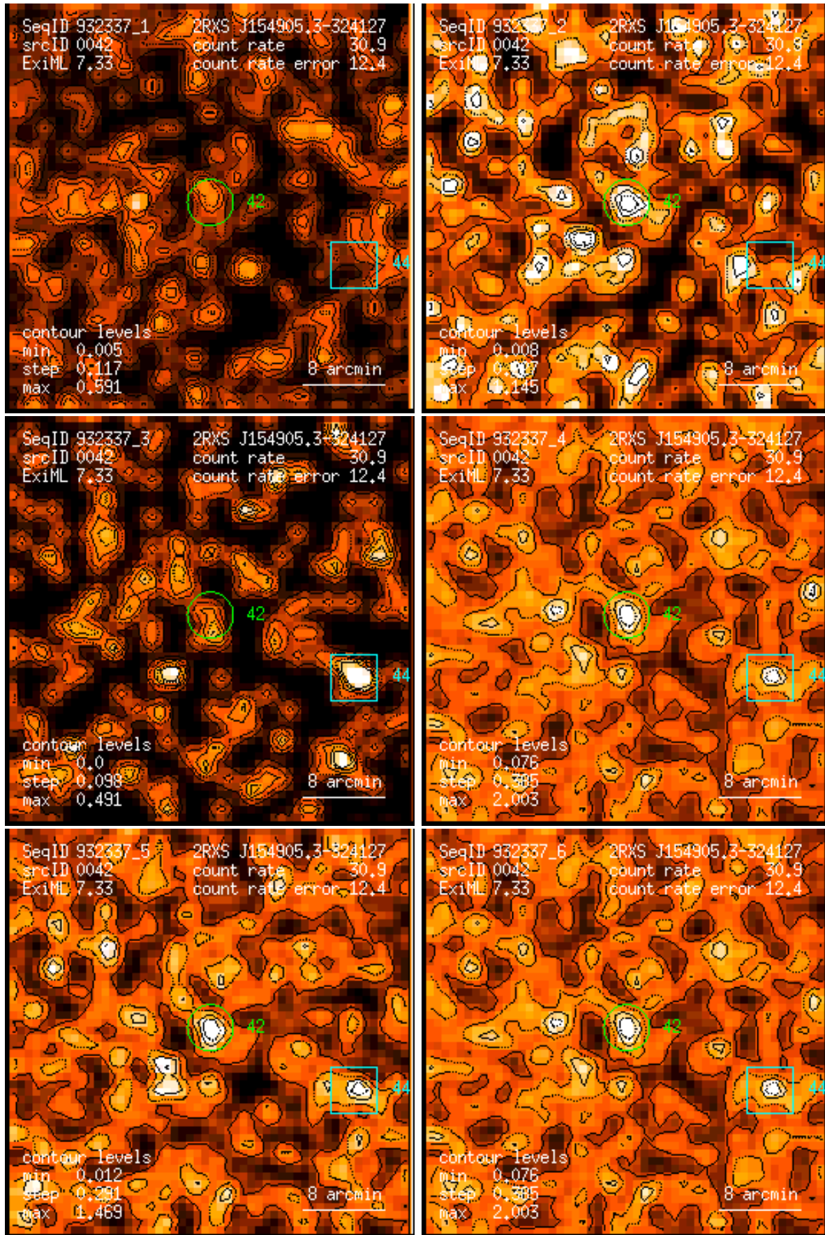
Figure 42: RASS 932337: detection 0042: band rate images, Gaussian filter: (1) PSPC channels 11 – 41, (2) 52 – 90, (3) 91 – 201, (4) 11 – 235, (5) 52 – 201, (6) 11 – 201. Broad band rates in counts/ks. Band rate contour levels in counts/ks/arcmin 2 .
