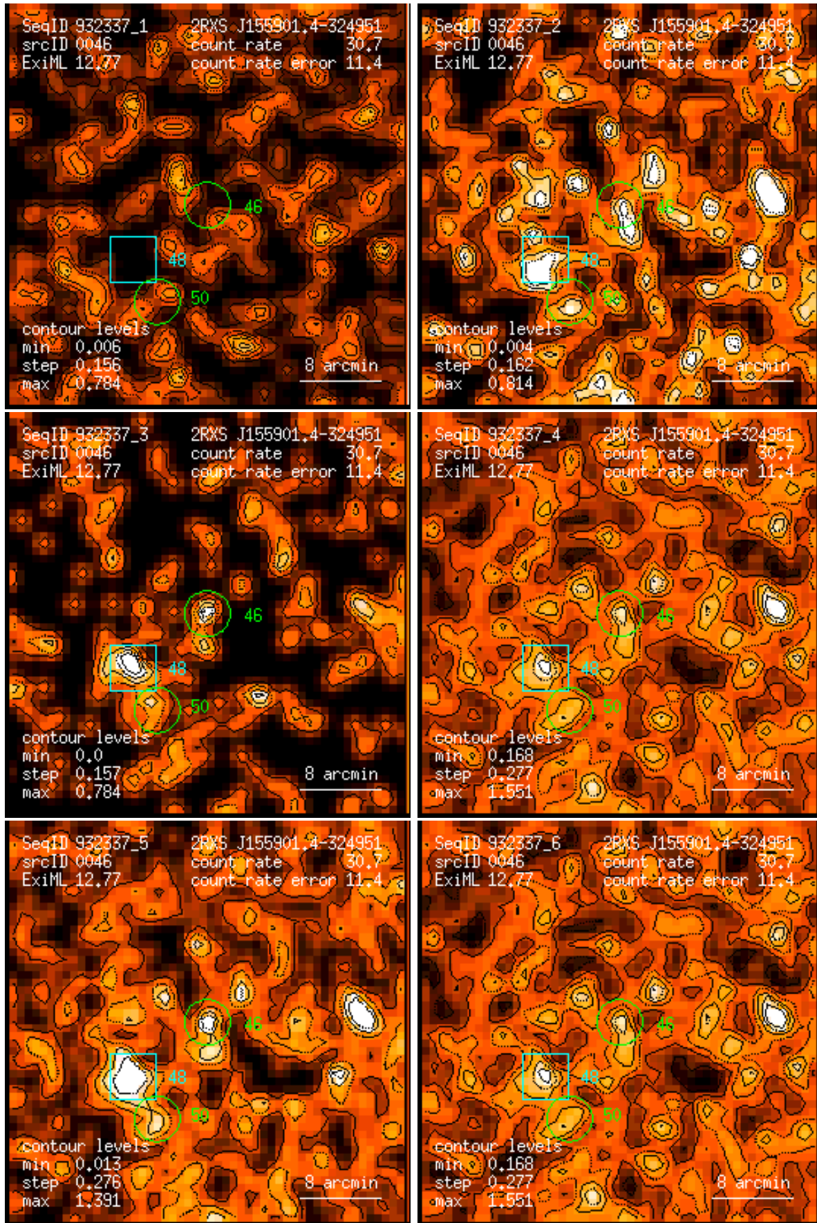
Figure 46: RASS 932337: detection 0046: band rate images, Gaussian filter: (1) PSPC channels 11 – 41, (2) 52 – 90, (3) 91 – 201, (4) 11 – 235, (5) 52 – 201, (6) 11 – 201. Broad band rates in counts/ks. Band rate contour levels in counts/ks/arcmin 2 .
