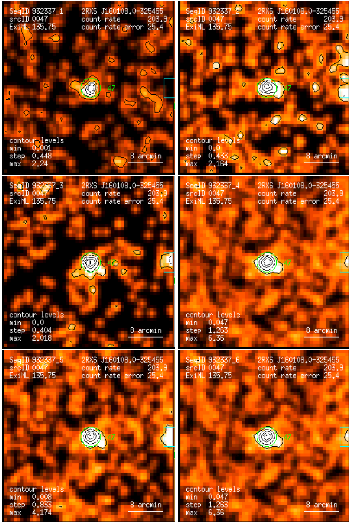
Figure 47: RASS 932337: detection 0047: band rate images, Gaussian filter: (1) PSPC channels 11 – 41, (2) 52 – 90, (3) 91 – 201, (4) 11 – 235, (5) 52 – 201, (6) 11 – 201. Broad band rates in counts/ks. Band rate contour levels in counts/ks/arcmin 2 .
