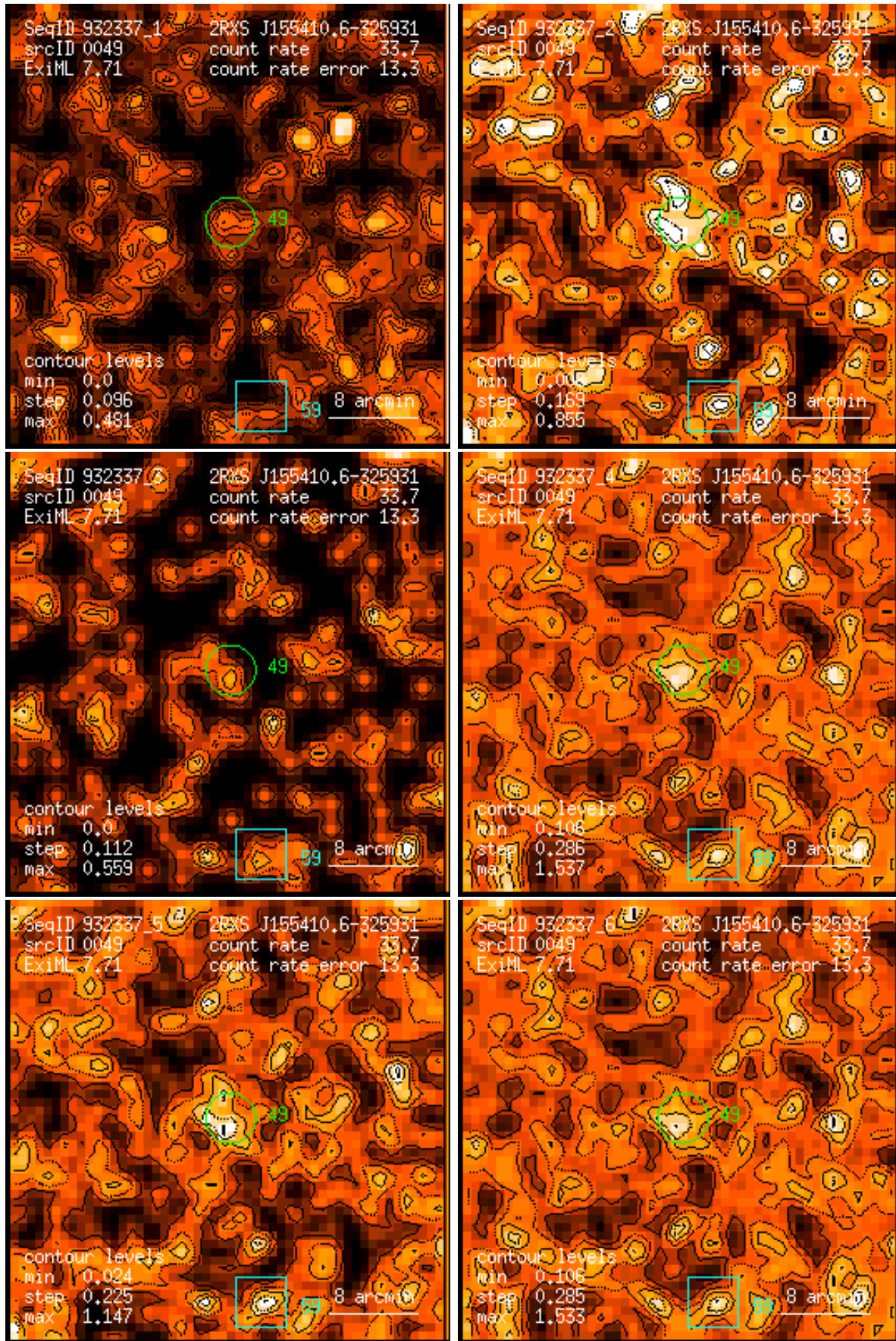
Figure 49: RASS 932337: detection 0049: band rate images, Gaussian filter: (1) PSPC channels 11 – 41, (2) 52 – 90, (3) 91 – 201, (4) 11 – 235, (5) 52 – 201, (6) 11 – 201. Broad band rates in counts/ks. Band rate contour levels in counts/ks/arcmin 2 .
