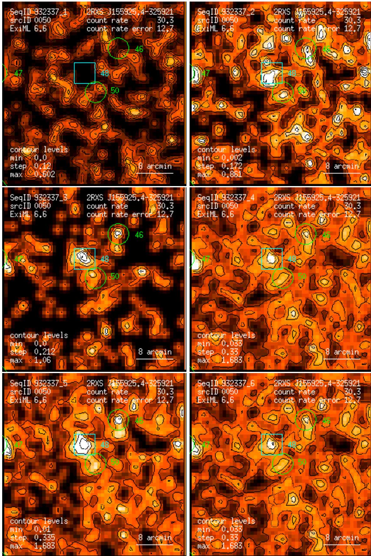
Figure 50: RASS 932337: detection 0050: band rate images, Gaussian filter: (1) PSPC channels 11 – 41, (2) 52 – 90, (3) 91 – 201, (4) 11 – 235, (5) 52 – 201, (6) 11 – 201. Broad band rates in counts/ks. Band rate contour levels in counts/ks/arcmin 2 .
