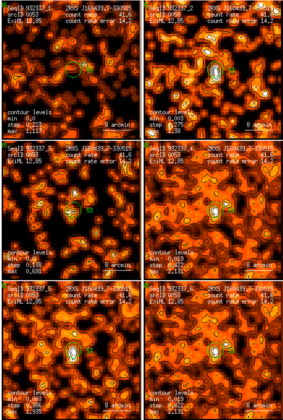
Figure 53: RASS 932337: detection 0053: band rate images, Gaussian filter: (1) PSPC channels 11 – 41, (2) 52 – 90, (3) 91 – 201, (4) 11 – 235, (5) 52 – 201, (6) 11 – 201. Broad band rates in counts/ks. Band rate contour levels in counts/ks/arcmin 2 .
