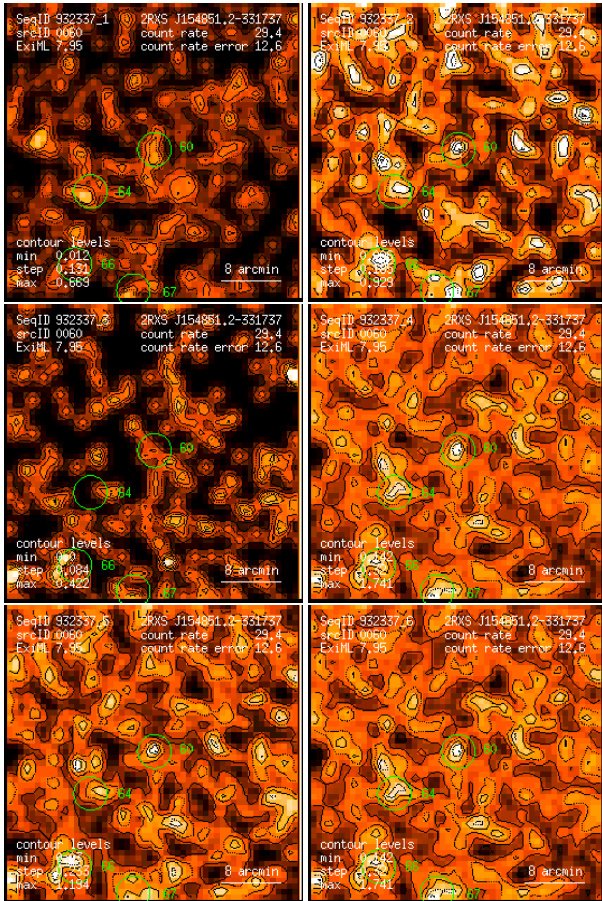
Figure 60: RASS 932337: detection 0060: band rate images, Gaussian filter: (1) PSPC channels 11 – 41, (2) 52 – 90, (3) 91 – 201, (4) 11 – 235, (5) 52 – 201, (6) 11 – 201. Broad band rates in counts/ks. Band rate contour levels in counts/ks/arcmin 2 .
