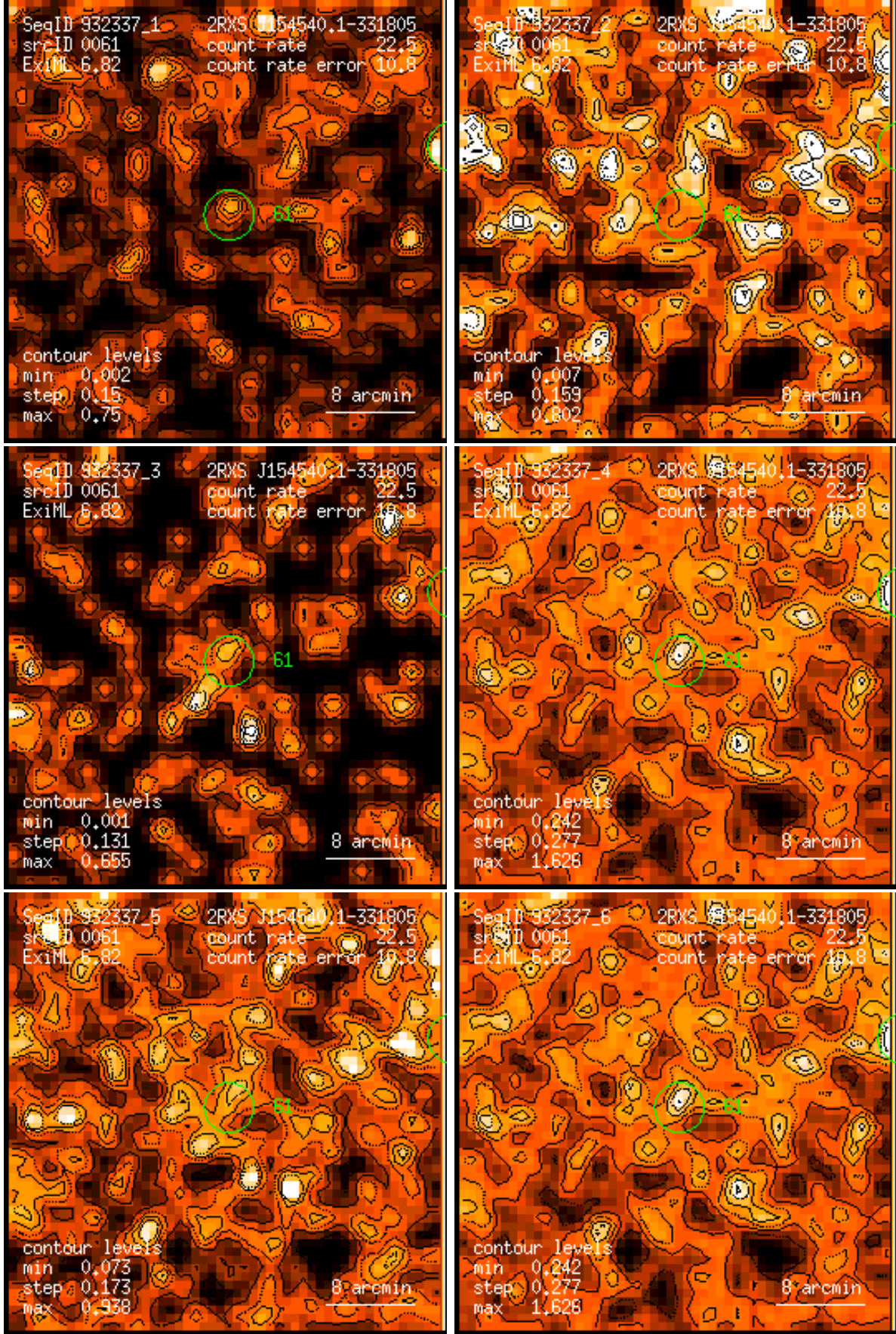
Figure 61: RASS 932337: detection 0061: band rate images, Gaussian filter: (1) PSPC channels 11 – 41, (2) 52 – 90, (3) 91 – 201, (4) 11 – 235, (5) 52 – 201, (6) 11 – 201. Broad band rates in counts/ks. Band rate contour levels in counts/ks/arcmin 2 .
