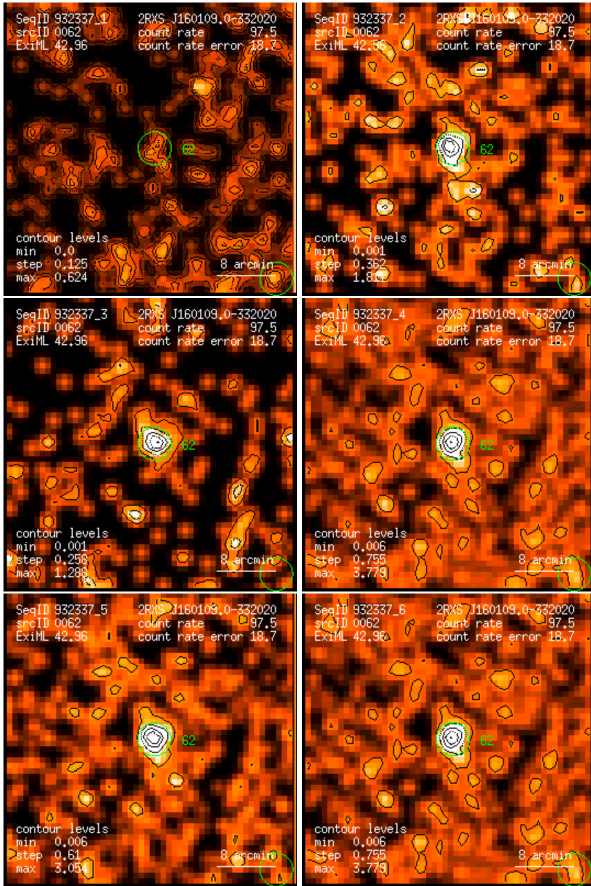
Figure 62: RASS 932337: detection 0062: band rate images, Gaussian filter: (1) PSPC channels 11 – 41, (2) 52 – 90, (3) 91 – 201, (4) 11 – 235, (5) 52 – 201, (6) 11 – 201. Broad band rates in counts/ks. Band rate contour levels in counts/ks/arcmin 2 .
