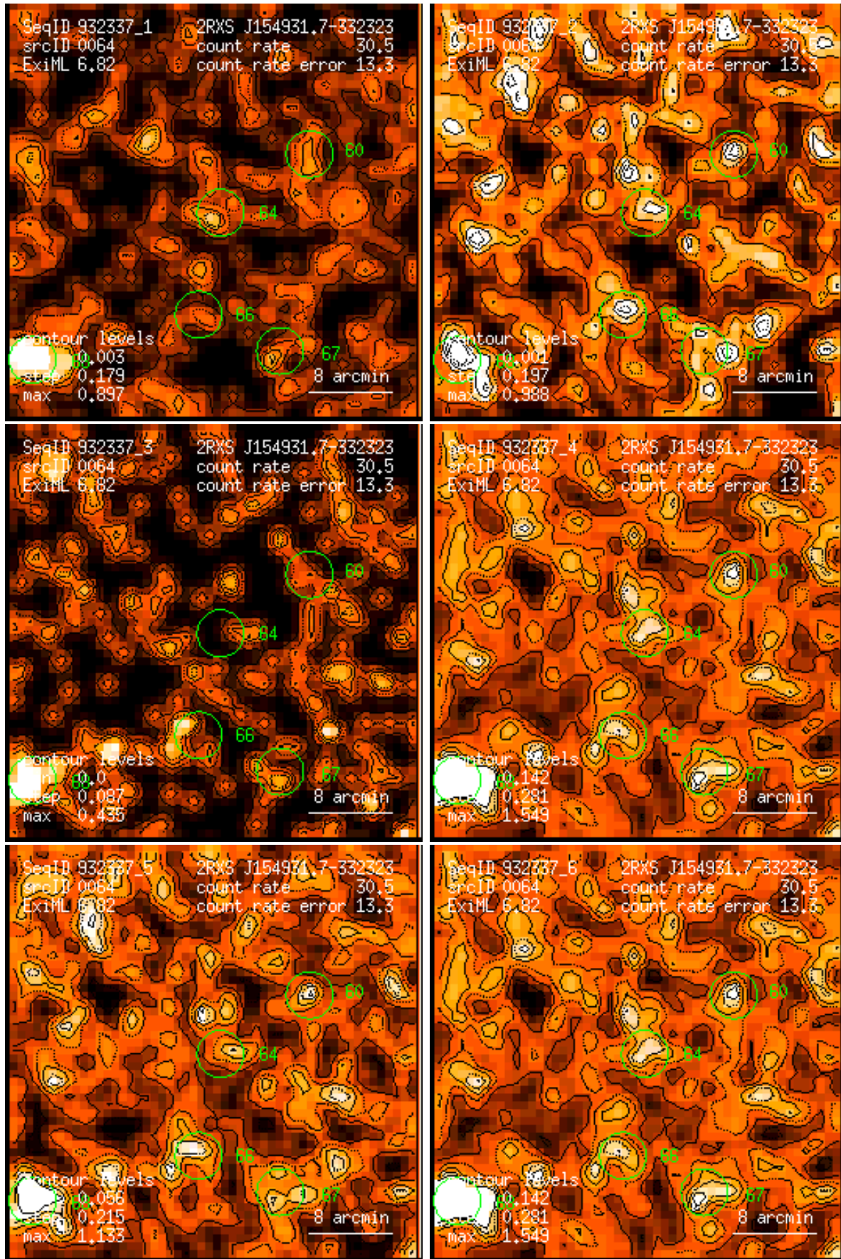
Figure 64: RASS 932337: detection 0064: band rate images, Gaussian filter: (1) PSPC channels 11 – 41, (2) 52 – 90, (3) 91 – 201, (4) 11 – 235, (5) 52 – 201, (6) 11 – 201. Broad band rates in counts/ks. Band rate contour levels in counts/ks/arcmin 2 .
