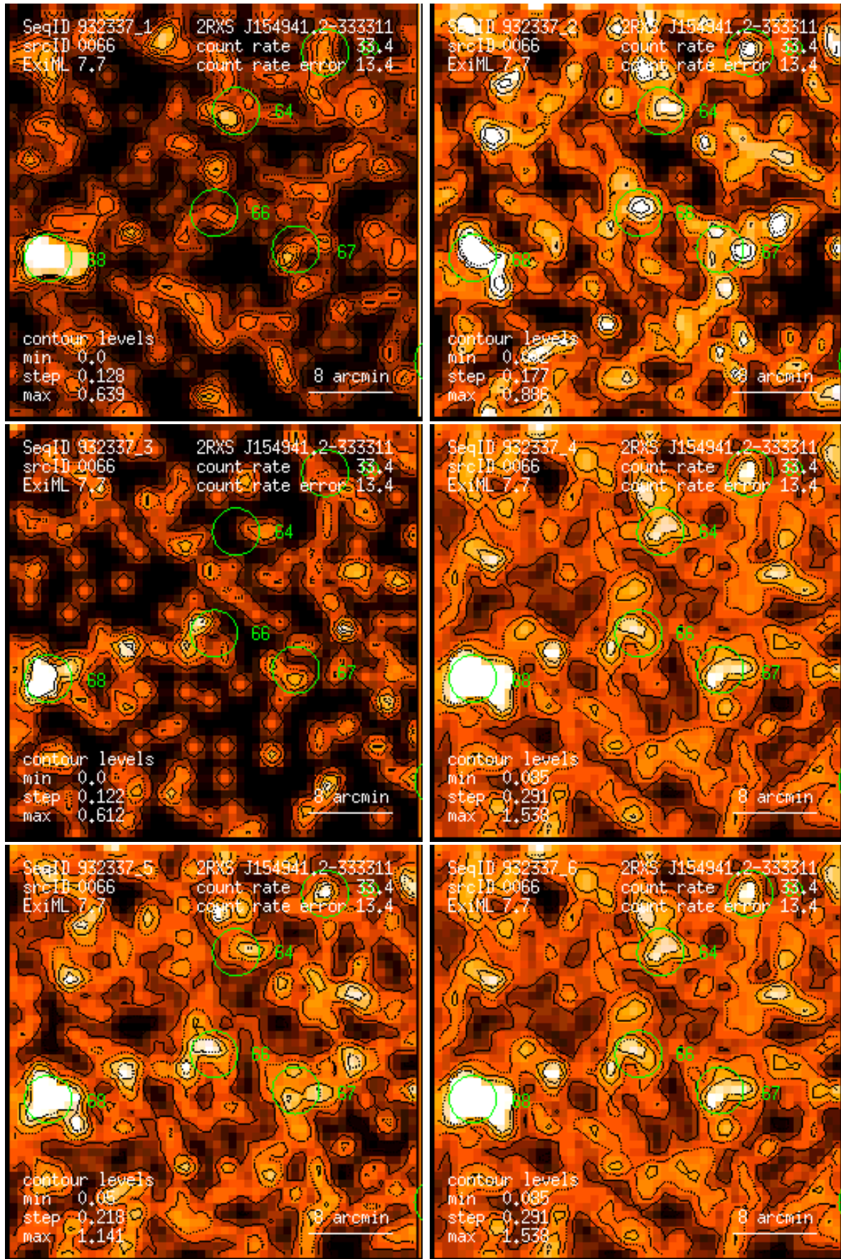
Figure 66: RASS 932337: detection 0066: band rate images, Gaussian filter: (1) PSPC channels 11 – 41, (2) 52 – 90, (3) 91 – 201, (4) 11 – 235, (5) 52 – 201, (6) 11 – 201. Broad band rates in counts/ks. Band rate contour levels in counts/ks/arcmin 2 .
