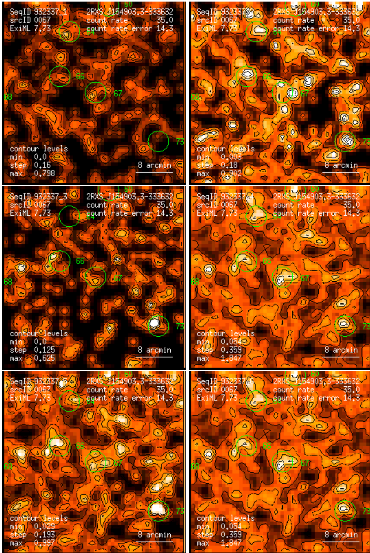
Figure 67: RASS 932337: detection 0067: band rate images, Gaussian filter: (1) PSPC channels 11 – 41, (2) 52 – 90, (3) 91 – 201, (4) 11 – 235, (5) 52 – 201, (6) 11 – 201. Broad band rates in counts/ks. Band rate contour levels in counts/ks/arcmin 2 .
