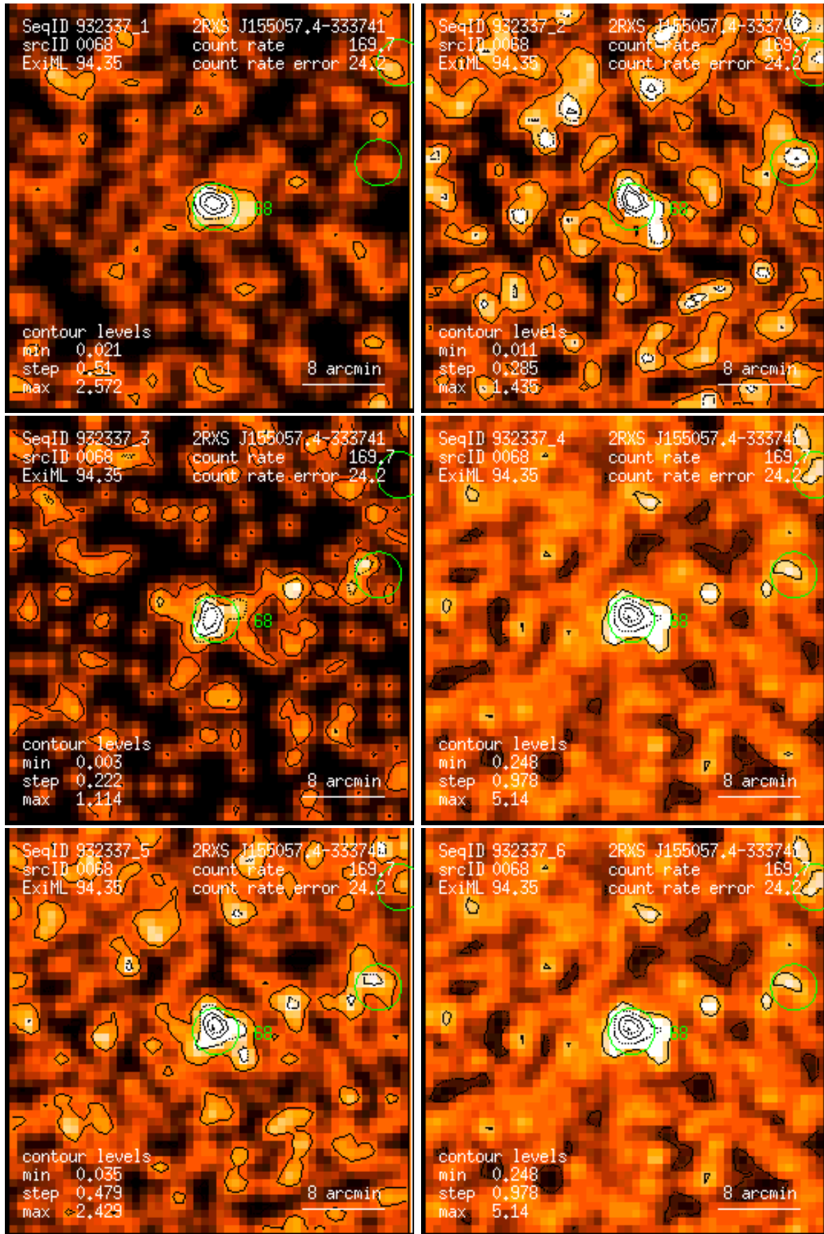
Figure 68: RASS 932337: detection 0068: band rate images, Gaussian filter: (1) PSPC channels 11 – 41, (2) 52 – 90, (3) 91 – 201, (4) 11 – 235, (5) 52 – 201, (6) 11 – 201. Broad band rates in counts/ks. Band rate contour levels in counts/ks/arcmin 2 .
