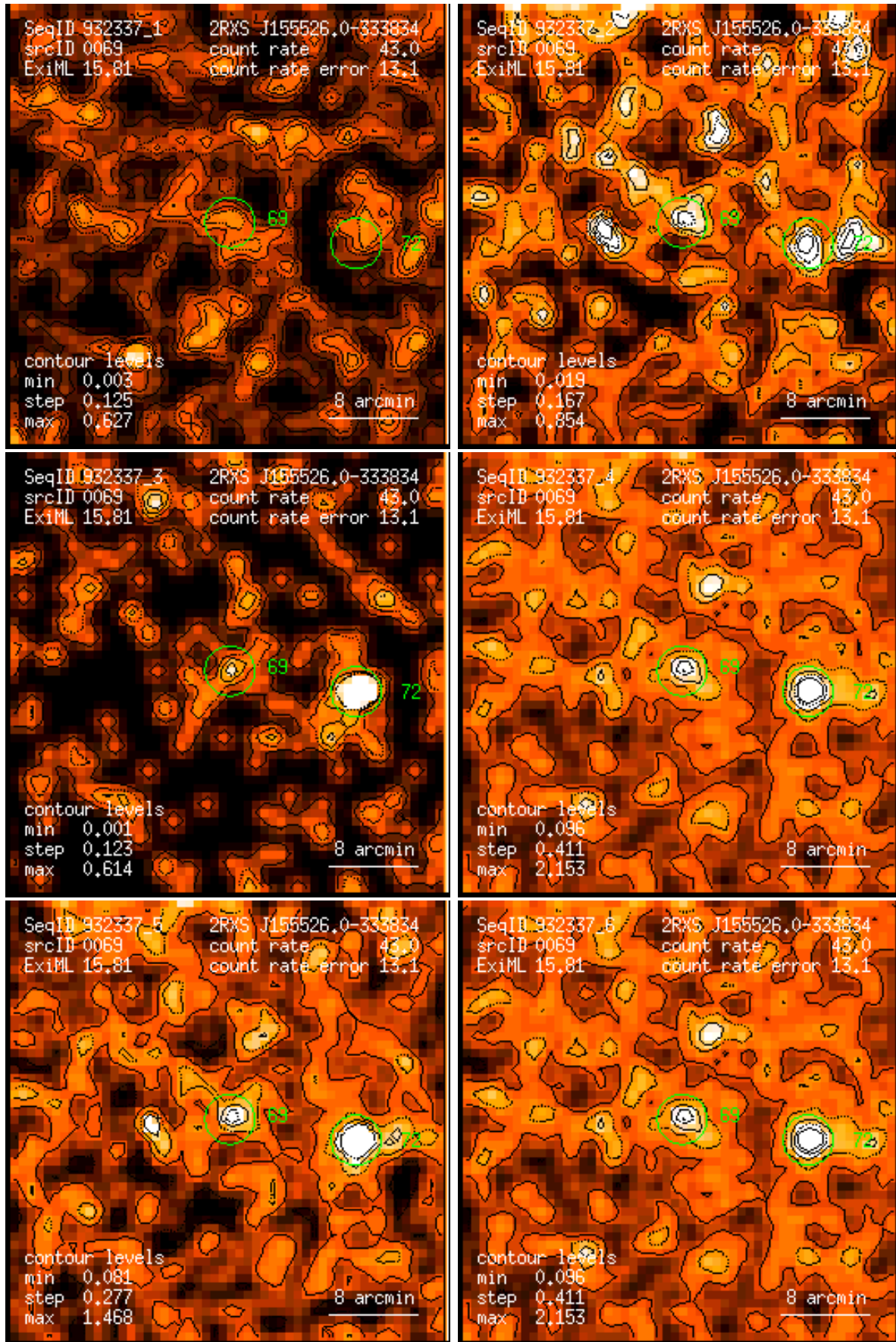
Figure 69: RASS 932337: detection 0069: band rate images, Gaussian filter: (1) PSPC channels 11 – 41, (2) 52 – 90, (3) 91 – 201, (4) 11 – 235, (5) 52 – 201, (6) 11 – 201. Broad band rates in counts/ks. Band rate contour levels in counts/ks/arcmin 2 .
