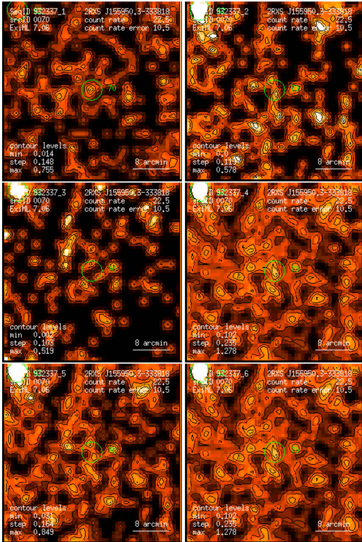
Figure 70: RASS 932337: detection 0070: band rate images, Gaussian filter: (1) PSPC channels 11 – 41, (2) 52 – 90, (3) 91 – 201, (4) 11 – 235, (5) 52 – 201, (6) 11 – 201. Broad band rates in counts/ks. Band rate contour levels in counts/ks/arcmin 2 .
