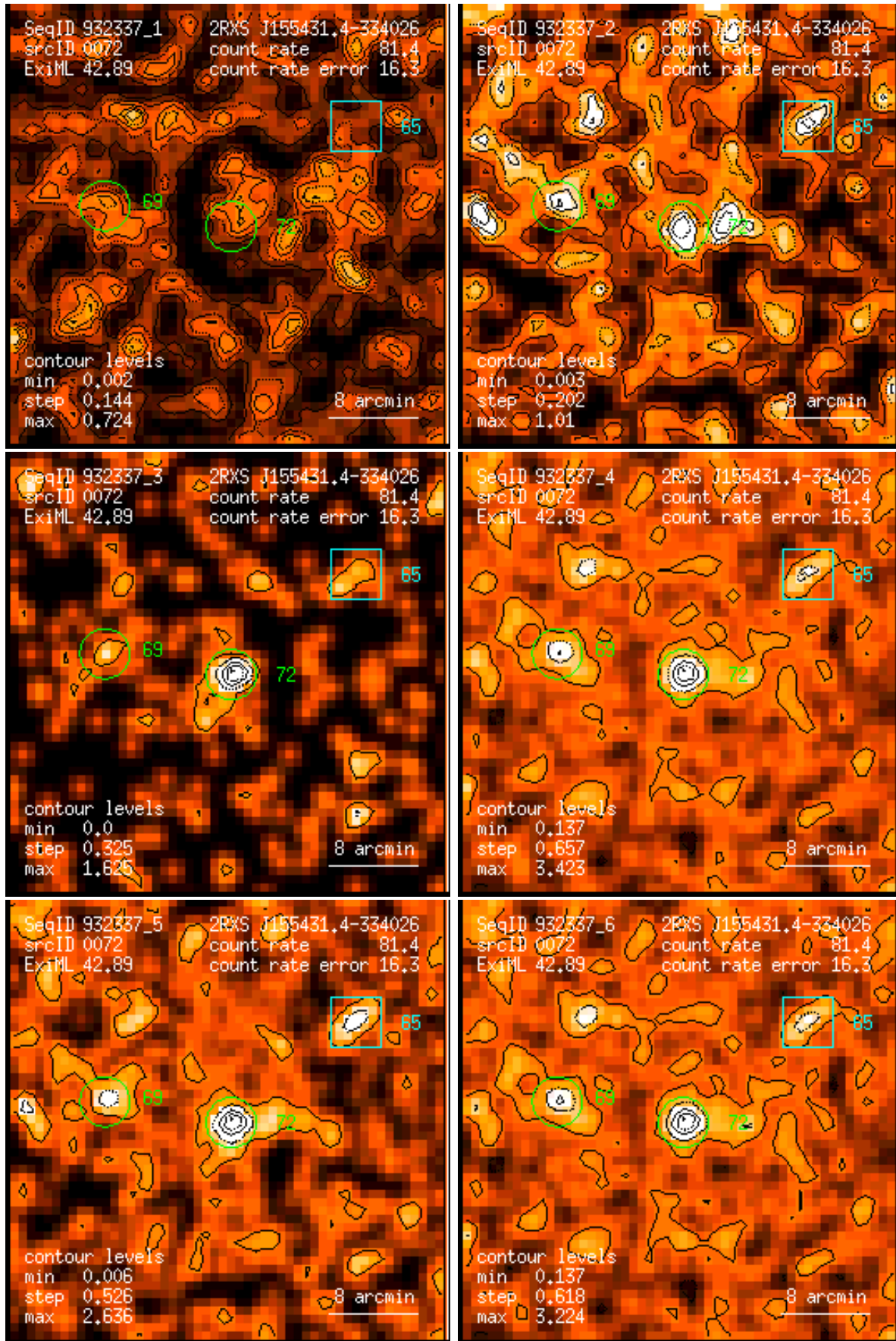
Figure 72: RASS 932337: detection 0072: band rate images, Gaussian filter: (1) PSPC channels 11 – 41, (2) 52 – 90, (3) 91 – 201, (4) 11 – 235, (5) 52 – 201, (6) 11 – 201. Broad band rates in counts/ks. Band rate contour levels in counts/ks/arcmin 2 .
