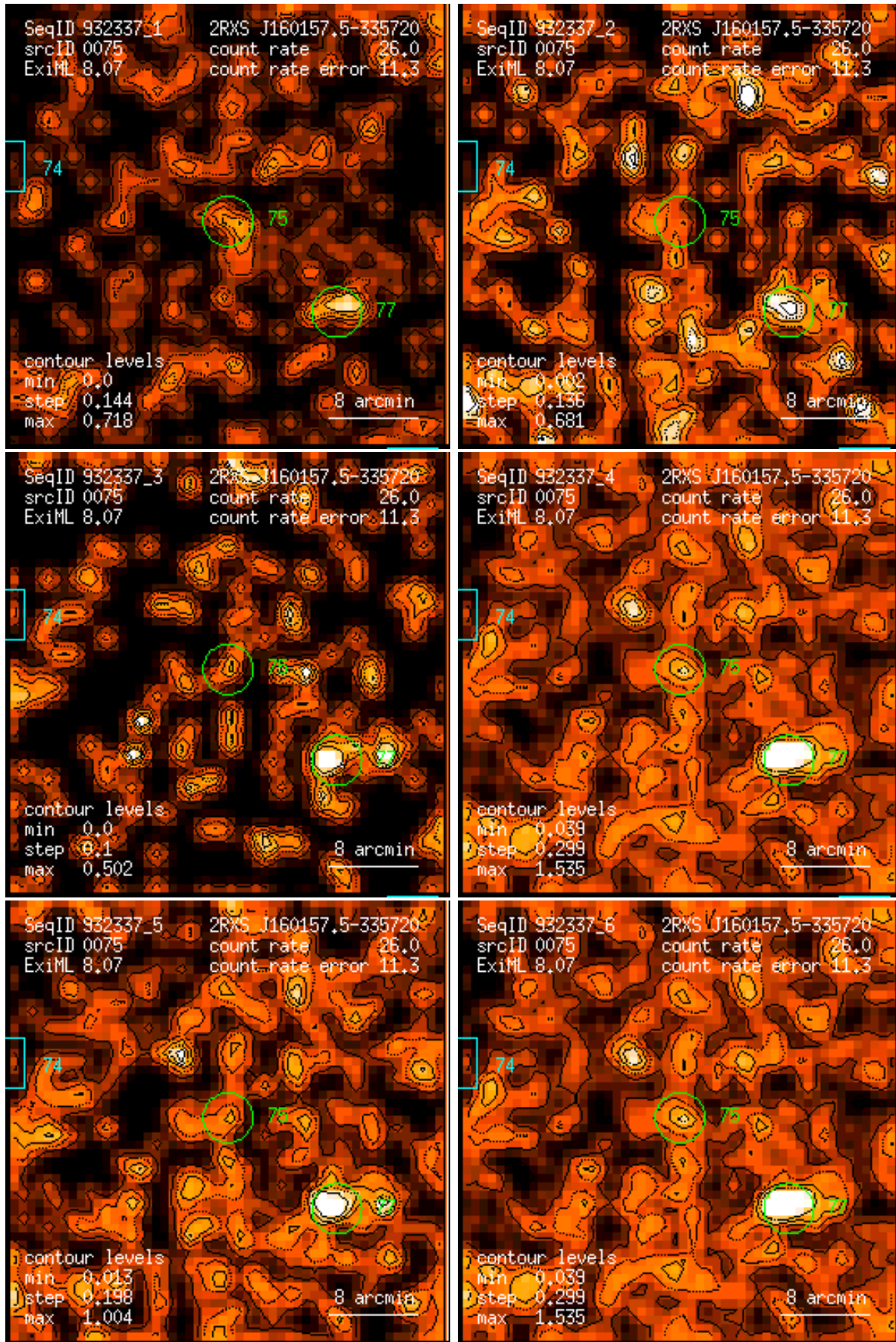
Figure 75: RASS 932337: detection 0075: band rate images, Gaussian filter: (1) PSPC channels 11 – 41, (2) 52 – 90, (3) 91 – 201, (4) 11 – 235, (5) 52 – 201, (6) 11 – 201. Broad band rates in counts/ks. Band rate contour levels in counts/ks/arcmin 2 .
