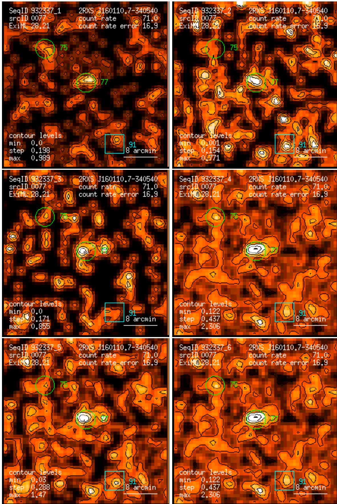
Figure 77: RASS 932337: detection 0077: band rate images, Gaussian filter: (1) PSPC channels 11 – 41, (2) 52 – 90, (3) 91 – 201, (4) 11 – 235, (5) 52 – 201, (6) 11 – 201. Broad band rates in counts/ks. Band rate contour levels in counts/ks/arcmin 2 .
