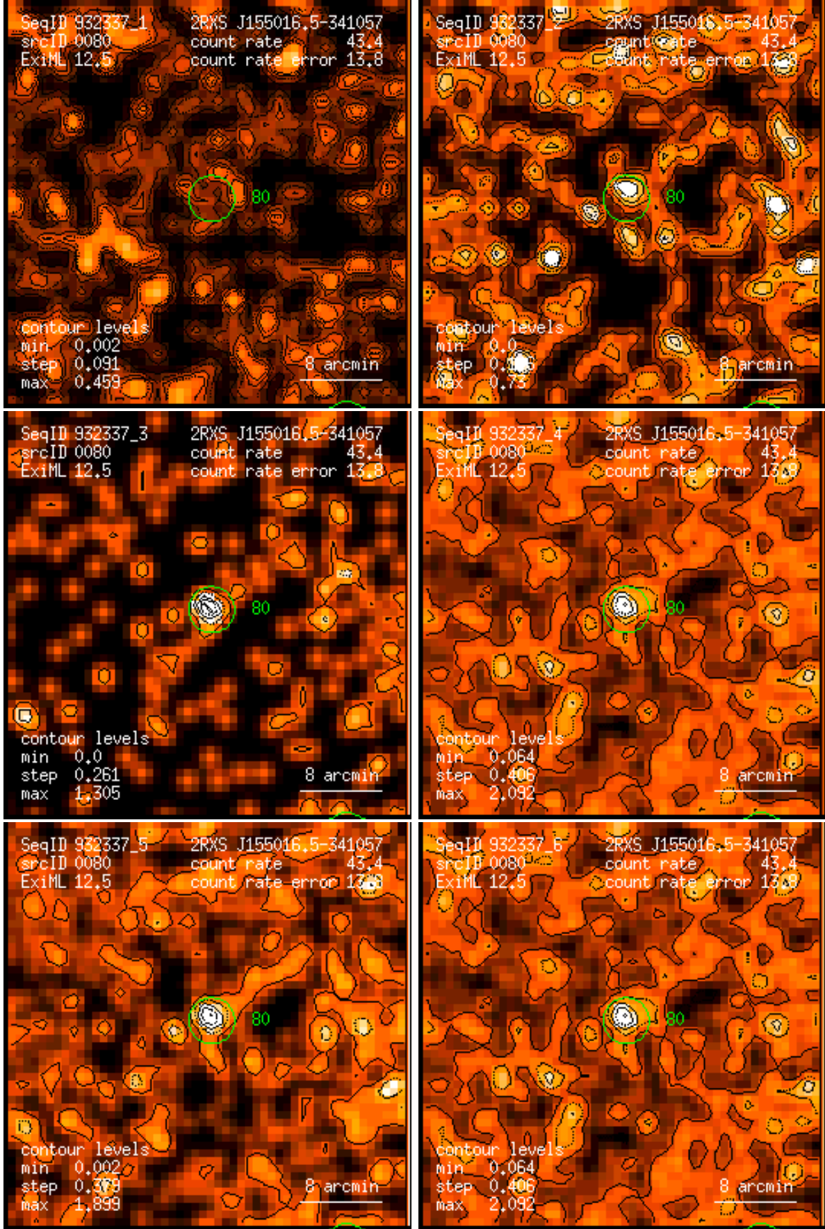
Figure 80: RASS 932337: detection 0080: band rate images, Gaussian filter: (1) PSPC channels 11 – 41, (2) 52 – 90, (3) 91 – 201, (4) 11 – 235, (5) 52 – 201, (6) 11 – 201. Broad band rates in counts/ks. Band rate contour levels in counts/ks/arcmin 2 .
