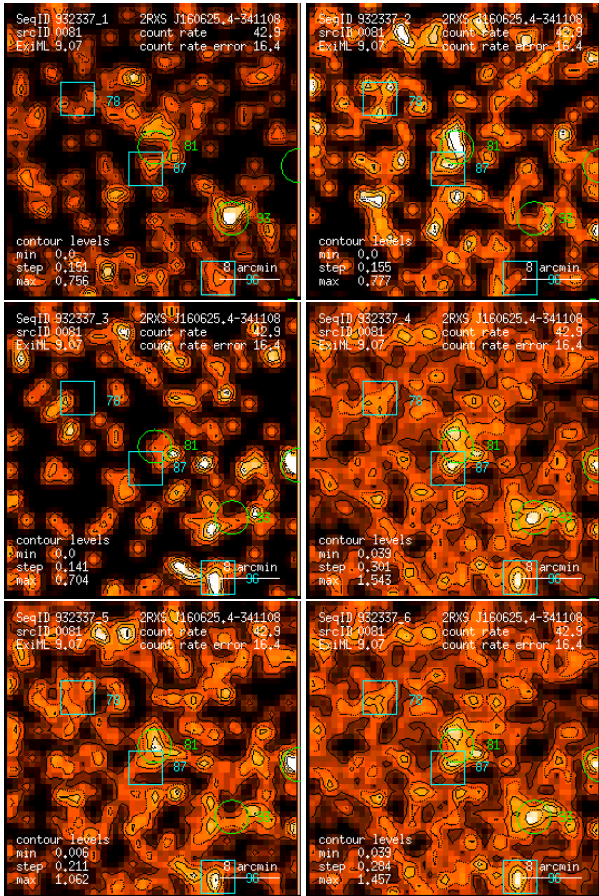
Figure 81: RASS 932337: detection 0081: band rate images, Gaussian filter: (1) PSPC channels 11 – 41, (2) 52 – 90, (3) 91 – 201, (4) 11 – 235, (5) 52 – 201, (6) 11 – 201. Broad band rates in counts/ks. Band rate contour levels in counts/ks/arcmin 2 .
