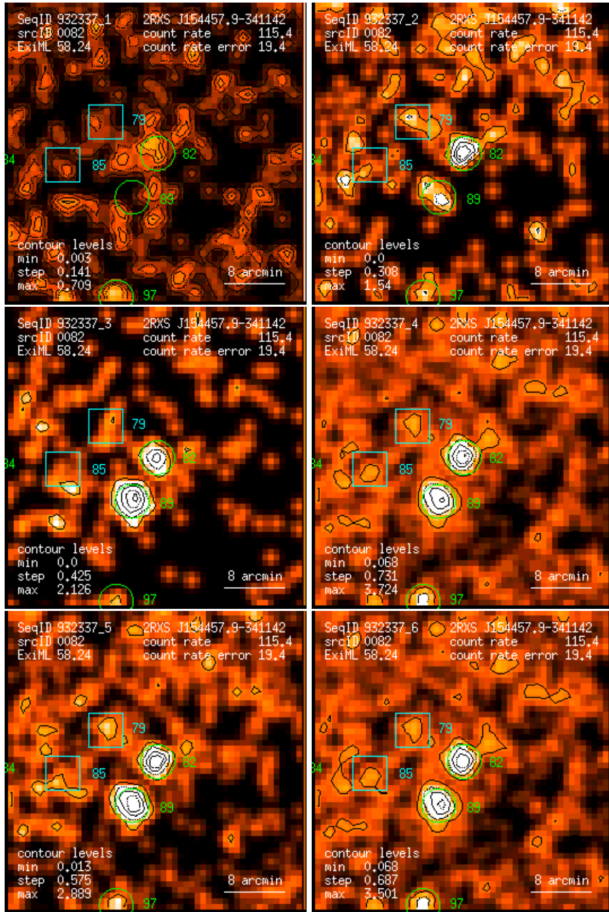
Figure 82: RASS 932337: detection 0082: band rate images, Gaussian filter: (1) PSPC channels 11 – 41, (2) 52 – 90, (3) 91 – 201, (4) 11 – 235, (5) 52 – 201, (6) 11 – 201. Broad band rates in counts/ks. Band rate contour levels in counts/ks/arcmin 2 .
