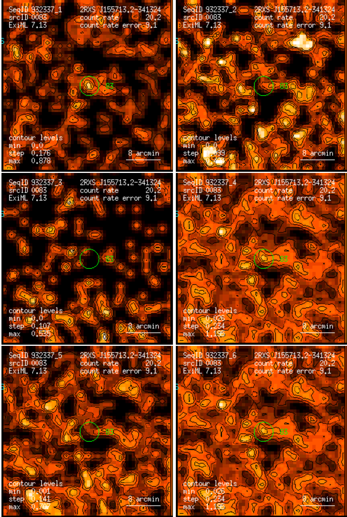
Figure 83: RASS 932337: detection 0083: band rate images, Gaussian filter: (1) PSPC channels 11 – 41, (2) 52 – 90, (3) 91 – 201, (4) 11 – 235, (5) 52 – 201, (6) 11 – 201. Broad band rates in counts/ks. Band rate contour levels in counts/ks/arcmin 2 .
