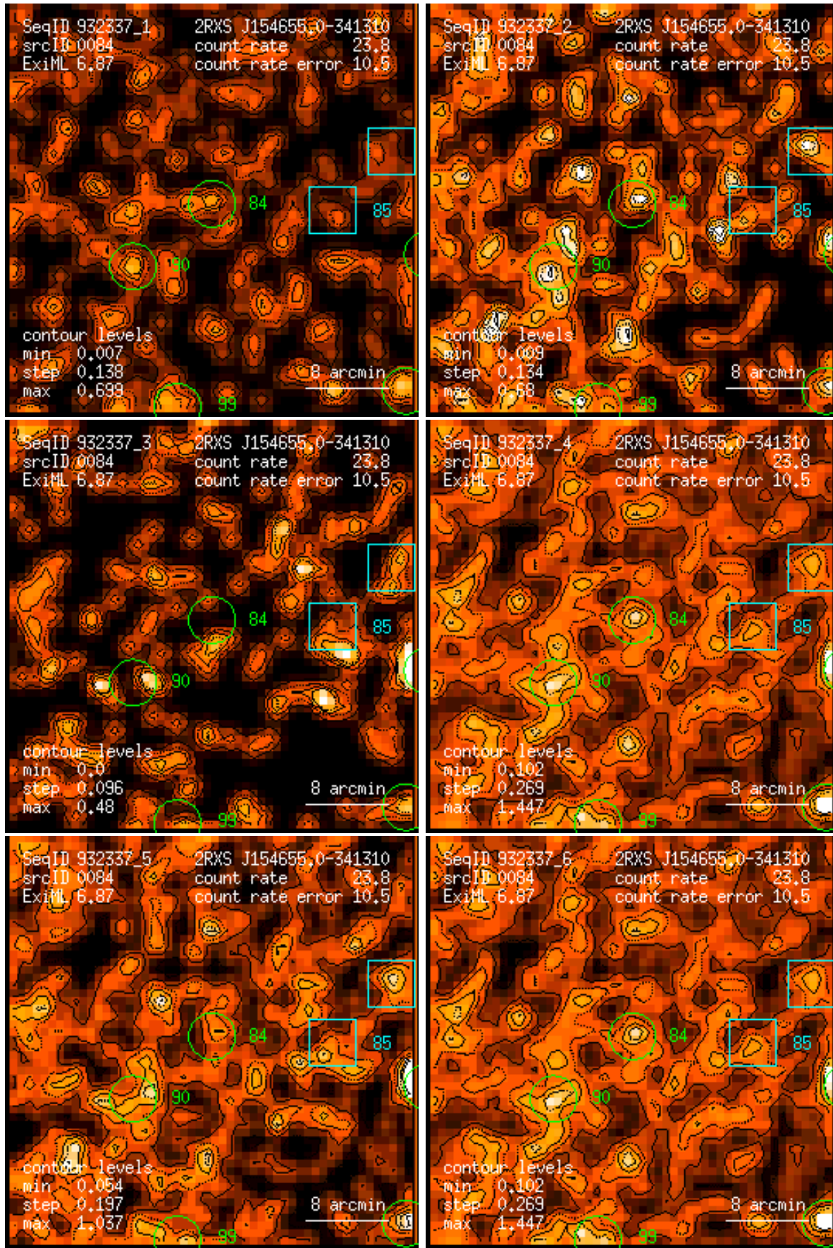
Figure 84: RASS 932337: detection 0084: band rate images, Gaussian filter: (1) PSPC channels 11 – 41, (2) 52 – 90, (3) 91 – 201, (4) 11 – 235, (5) 52 – 201, (6) 11 – 201. Broad band rates in counts/ks. Band rate contour levels in counts/ks/arcmin 2 .
