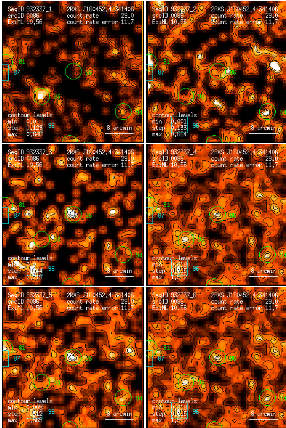
Figure 86: RASS 932337: detection 0086: band rate images, Gaussian filter: (1) PSPC channels 11 – 41, (2) 52 – 90, (3) 91 – 201, (4) 11 – 235, (5) 52 – 201, (6) 11 – 201. Broad band rates in counts/ks. Band rate contour levels in counts/ks/arcmin 2 .
