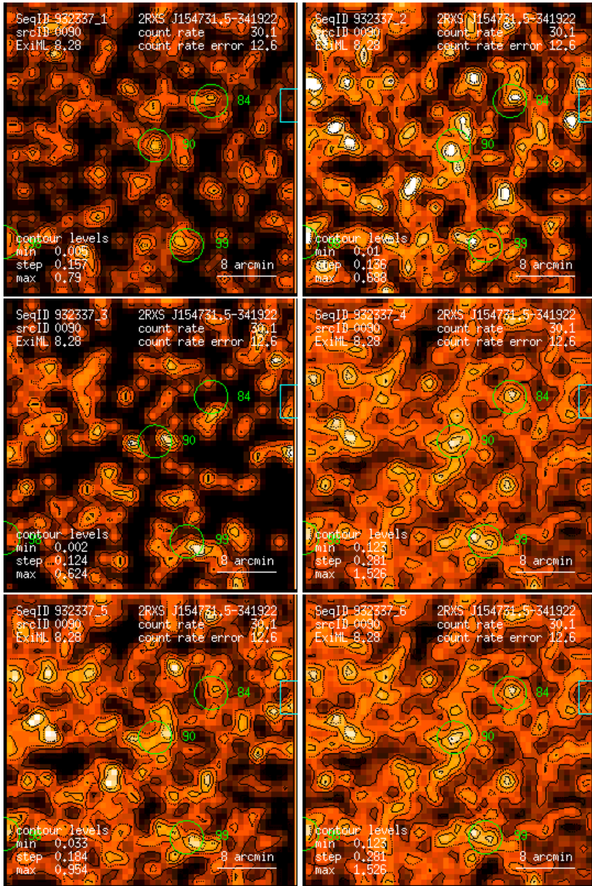
Figure 90: RASS 932337: detection 0090: band rate images, Gaussian filter: (1) PSPC channels 11 – 41, (2) 52 – 90, (3) 91 – 201, (4) 11 – 235, (5) 52 – 201, (6) 11 – 201. Broad band rates in counts/ks. Band rate contour levels in counts/ks/arcmin 2 .
