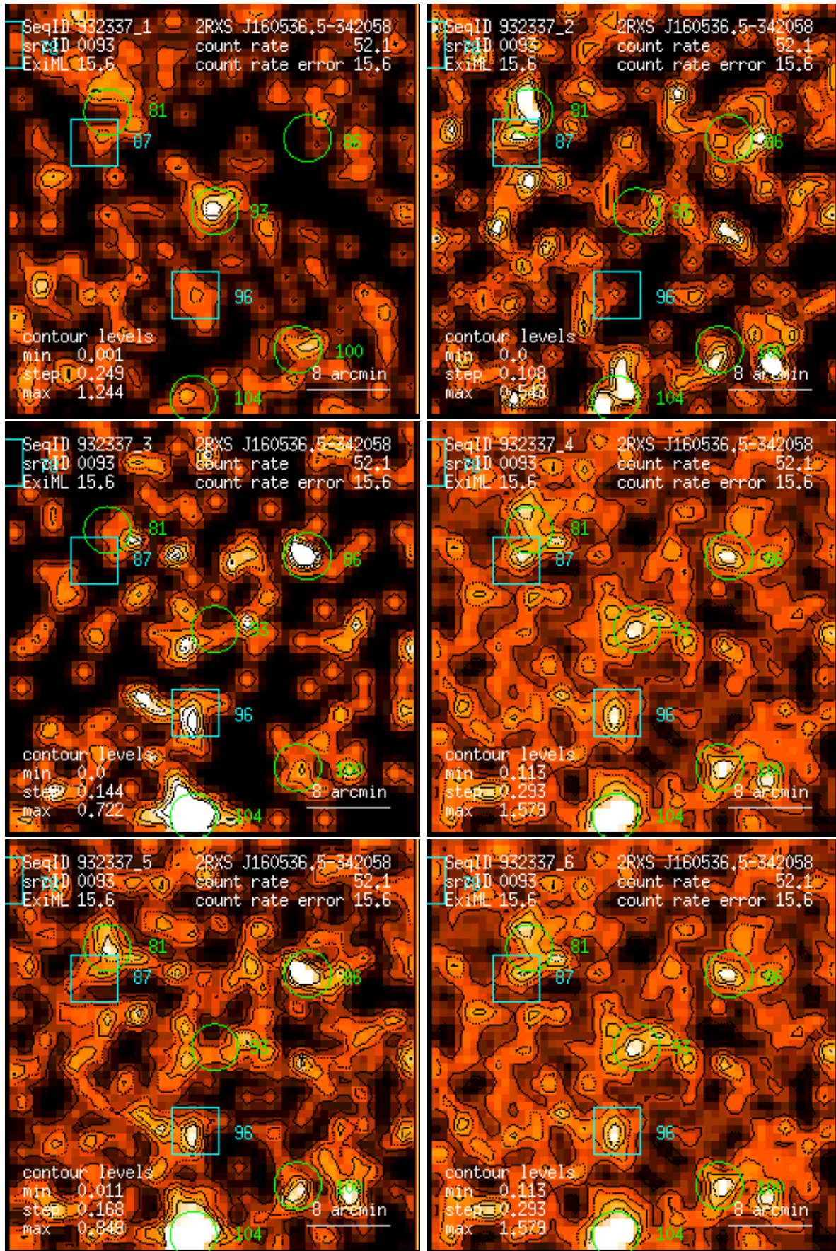
Figure 93: RASS 932337: detection 0093: band rate images, Gaussian filter: (1) PSPC channels 11 – 41, (2) 52 – 90, (3) 91 – 201, (4) 11 – 235, (5) 52 – 201, (6) 11 – 201. Broad band rates in counts/ks. Band rate contour levels in counts/ks/arcmin 2 .
