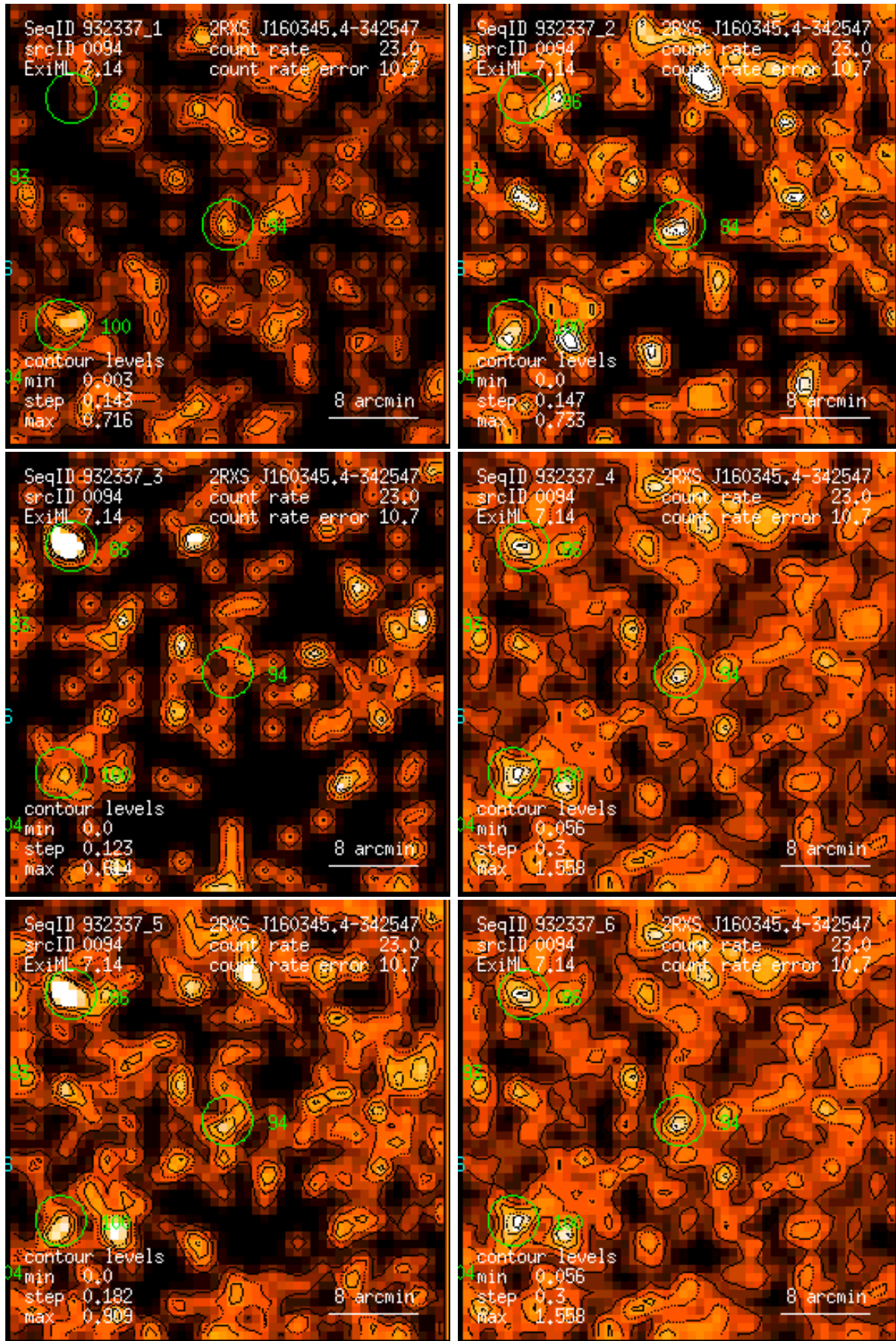
Figure 94: RASS 932337: detection 0094: band rate images, Gaussian filter: (1) PSPC channels 11 – 41, (2) 52 – 90, (3) 91 – 201, (4) 11 – 235, (5) 52 – 201, (6) 11 – 201. Broad band rates in counts/ks. Band rate contour levels in counts/ks/arcmin 2 .
