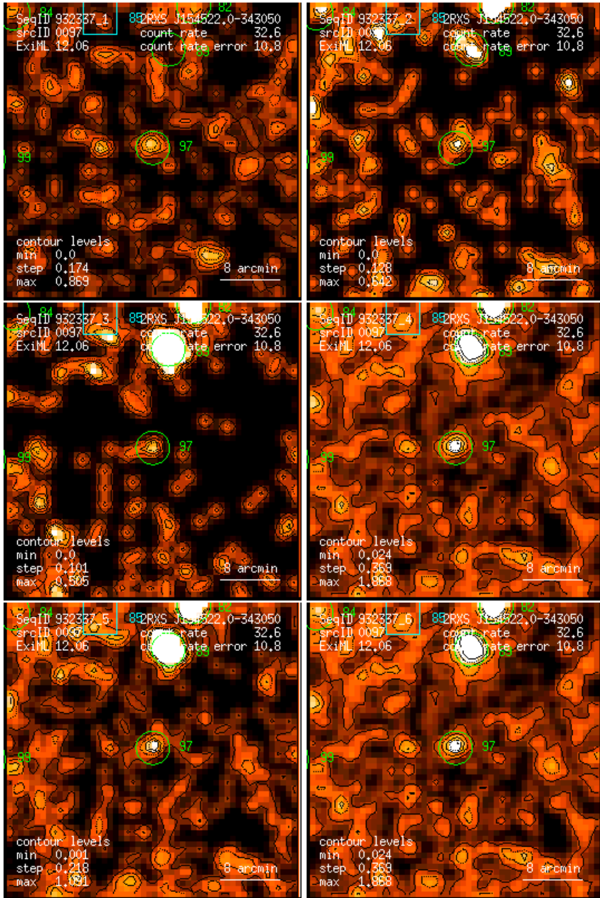
Figure 97: RASS 932337: detection 0097: band rate images, Gaussian filter: (1) PSPC channels 11 – 41, (2) 52 – 90, (3) 91 – 201, (4) 11 – 235, (5) 52 – 201, (6) 11 – 201. Broad band rates in counts/ks. Band rate contour levels in counts/ks/arcmin 2 .
