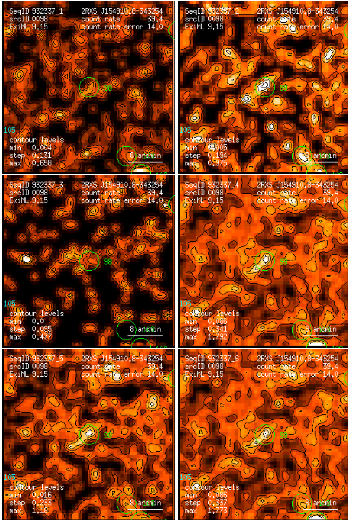
Figure 98: RASS 932337: detection 0098: band rate images, Gaussian filter: (1) PSPC channels 11 – 41, (2) 52 – 90, (3) 91 – 201, (4) 11 – 235, (5) 52 – 201, (6) 11 – 201. Broad band rates in counts/ks. Band rate contour levels in counts/ks/arcmin 2 .
