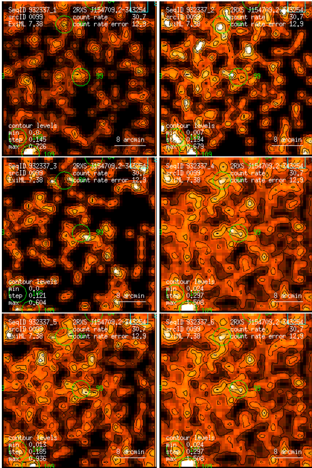
Figure 99: RASS 932337: detection 0099: band rate images, Gaussian filter: (1) PSPC channels 11 – 41, (2) 52 – 90, (3) 91 – 201, (4) 11 – 235, (5) 52 – 201, (6) 11 – 201. Broad band rates in counts/ks. Band rate contour levels in counts/ks/arcmin 2 .
