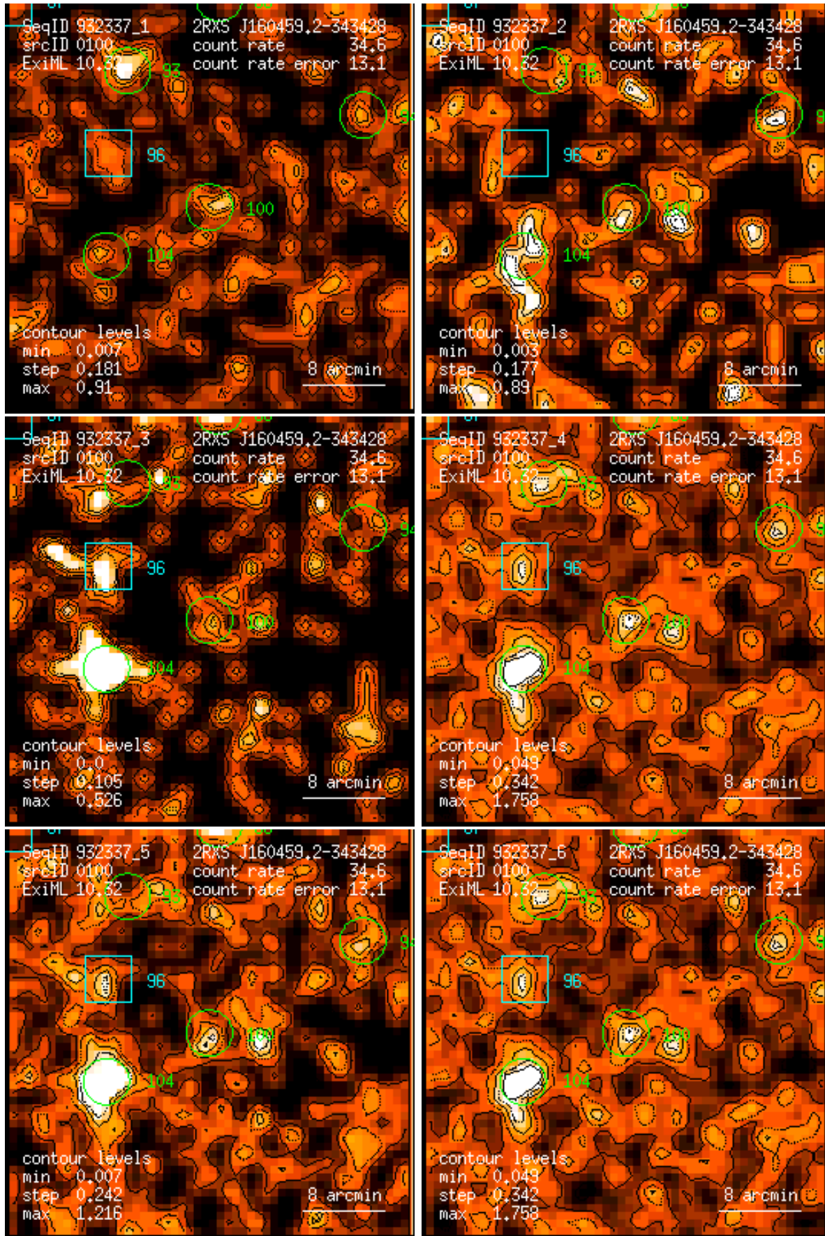
Figure 100: RASS 932337: detection 0100: band rate images, Gaussian filter: (1) PSPC channels 11 – 41, (2) 52 – 90, (3) 91 – 201, (4) 11 – 235, (5) 52 – 201, (6) 11 – 201. Broad band rates in counts/ks. Band rate contour levels in counts/ks/arcmin 2 .
