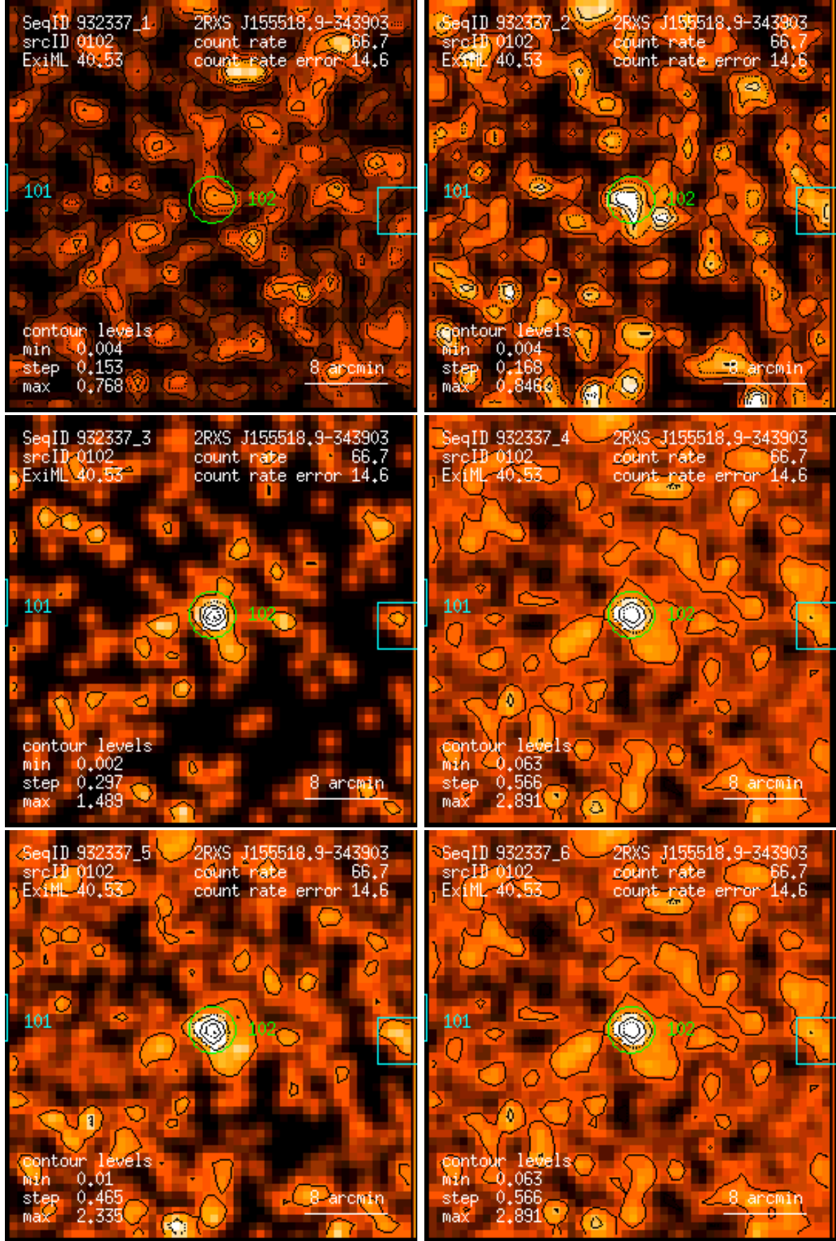
Figure 102: RASS 932337: detection 0102: band rate images, Gaussian filter: (1) PSPC channels 11 – 41, (2) 52 – 90, (3) 91 – 201, (4) 11 – 235, (5) 52 – 201, (6) 11 – 201. Broad band rates in counts/ks. Band rate contour levels in counts/ks/arcmin 2 .
