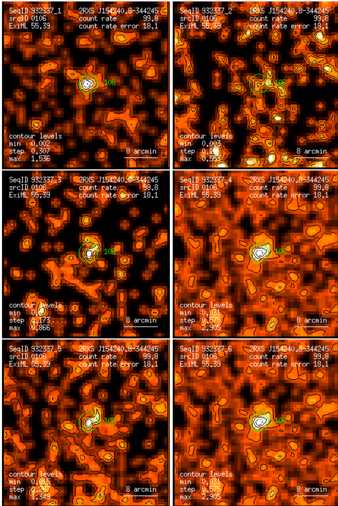
Figure 106: RASS 932337: detection 0106: band rate images, Gaussian filter: (1) PSPC channels 11 – 41, (2) 52 – 90, (3) 91 – 201, (4) 11 – 235, (5) 52 – 201, (6) 11 – 201. Broad band rates in counts/ks. Band rate contour levels in counts/ks/arcmin 2 .
