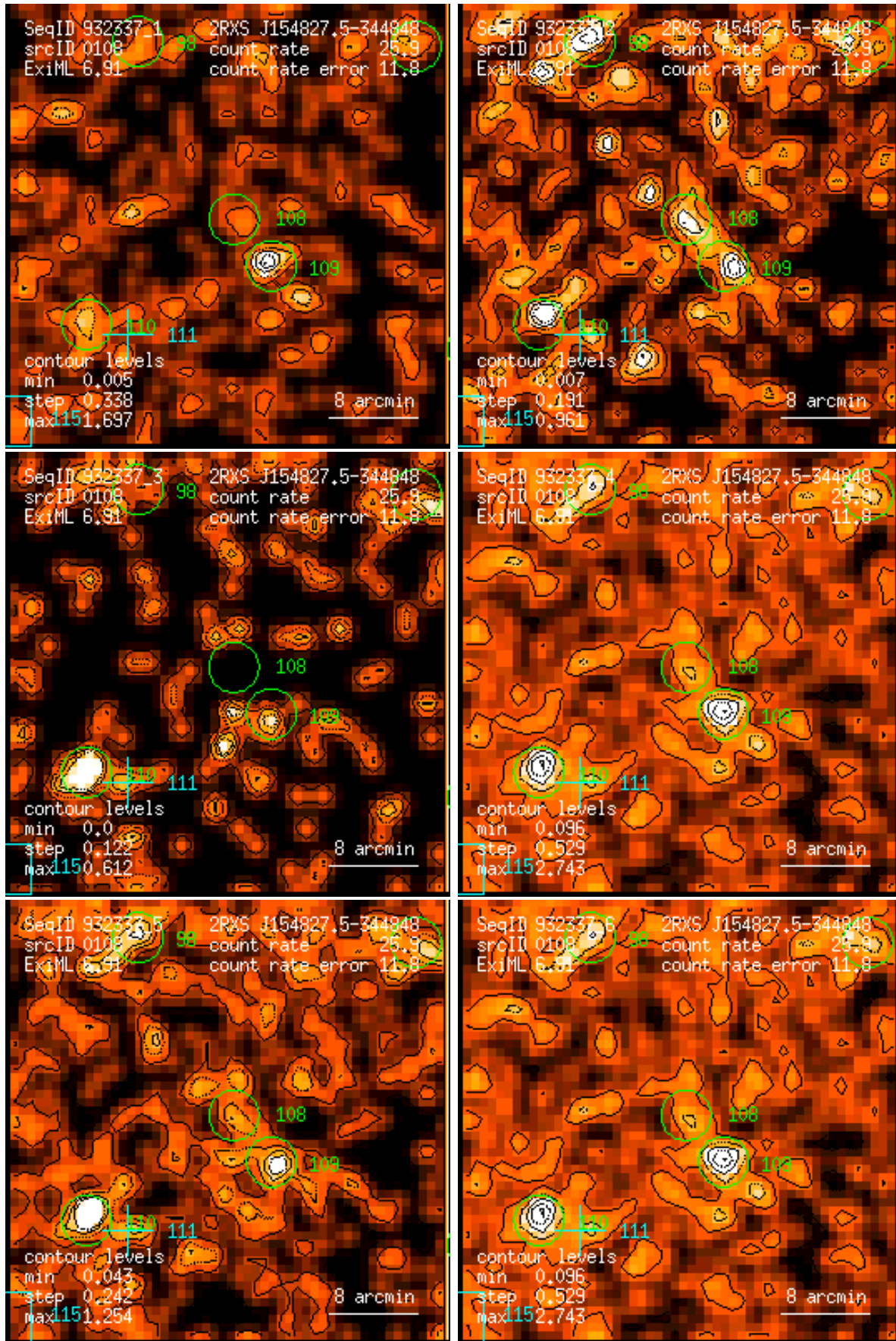
Figure 108: RASS 932337: detection 0108: band rate images, Gaussian filter: (1) PSPC channels 11 – 41, (2) 52 – 90, (3) 91 – 201, (4) 11 – 235, (5) 52 – 201, (6) 11 – 201. Broad band rates in counts/ks. Band rate contour levels in counts/ks/arcmin 2 .
