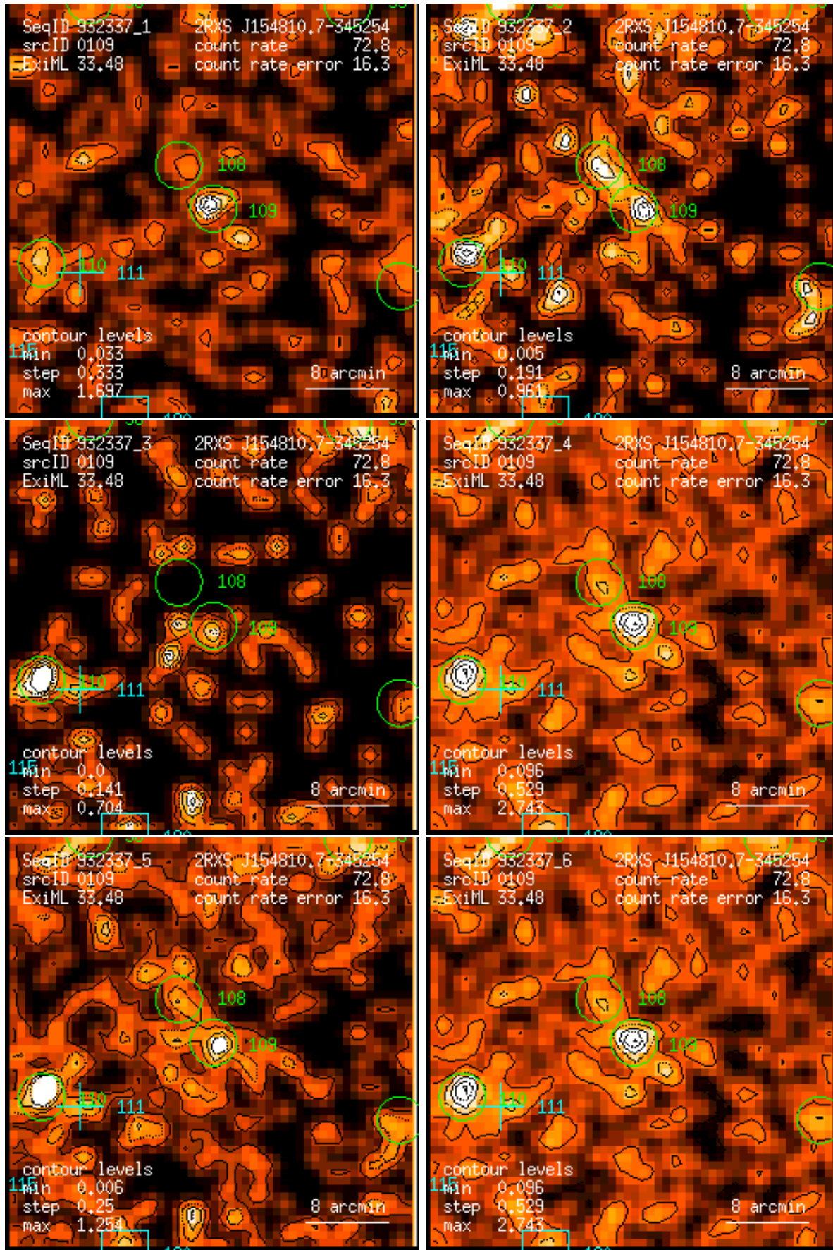
Figure 109: RASS 932337: detection 0109: band rate images, Gaussian filter: (1) PSPC channels 11 – 41, (2) 52 – 90, (3) 91 – 201, (4) 11 – 235, (5) 52 – 201, (6) 11 – 201. Broad band rates in counts/ks. Band rate contour levels in counts/ks/arcmin 2 .
