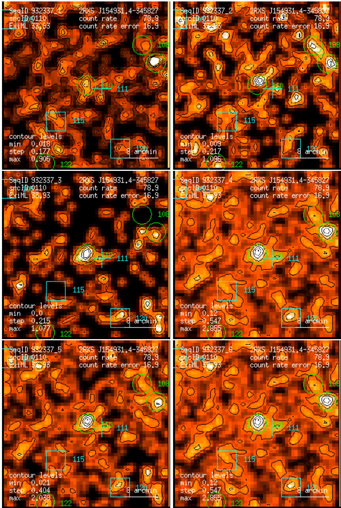
Figure 110: RASS 932337: detection 0110: band rate images, Gaussian filter: (1) PSPC channels 11 – 41, (2) 52 – 90, (3) 91 – 201, (4) 11 – 235, (5) 52 – 201, (6) 11 – 201. Broad band rates in counts/ks. Band rate contour levels in counts/ks/arcmin 2 .
