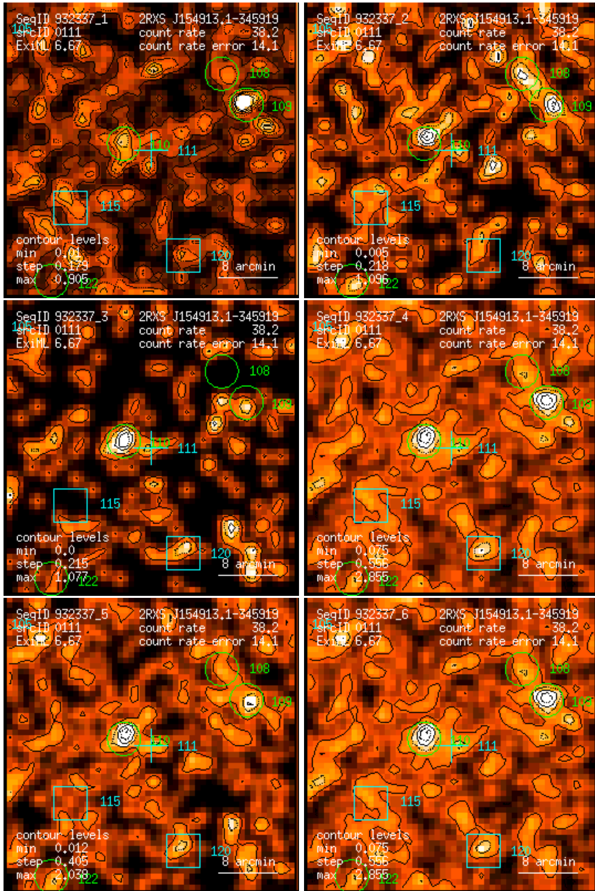
Figure 111: RASS 932337: detection 0111: band rate images, Gaussian filter: (1) PSPC channels 11 – 41, (2) 52 – 90, (3) 91 – 201, (4) 11 – 235, (5) 52 – 201, (6) 11 – 201. Broad band rates in counts/ks. Band rate contour levels in counts/ks/arcmin 2 .
