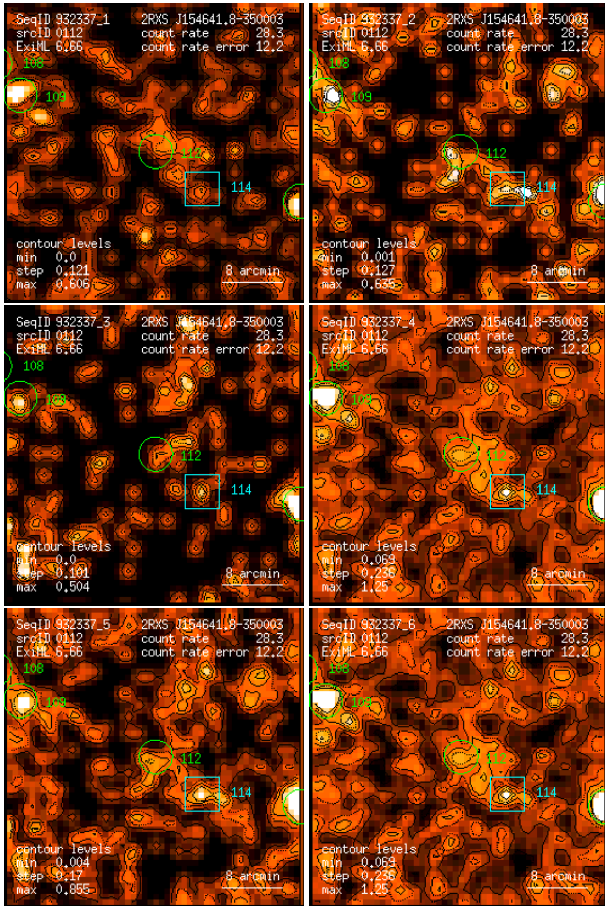
Figure 112: RASS 932337: detection 0112: band rate images, Gaussian filter: (1) PSPC channels 11 – 41, (2) 52 – 90, (3) 91 – 201, (4) 11 – 235, (5) 52 – 201, (6) 11 – 201. Broad band rates in counts/ks. Band rate contour levels in counts/ks/arcmin 2 .
