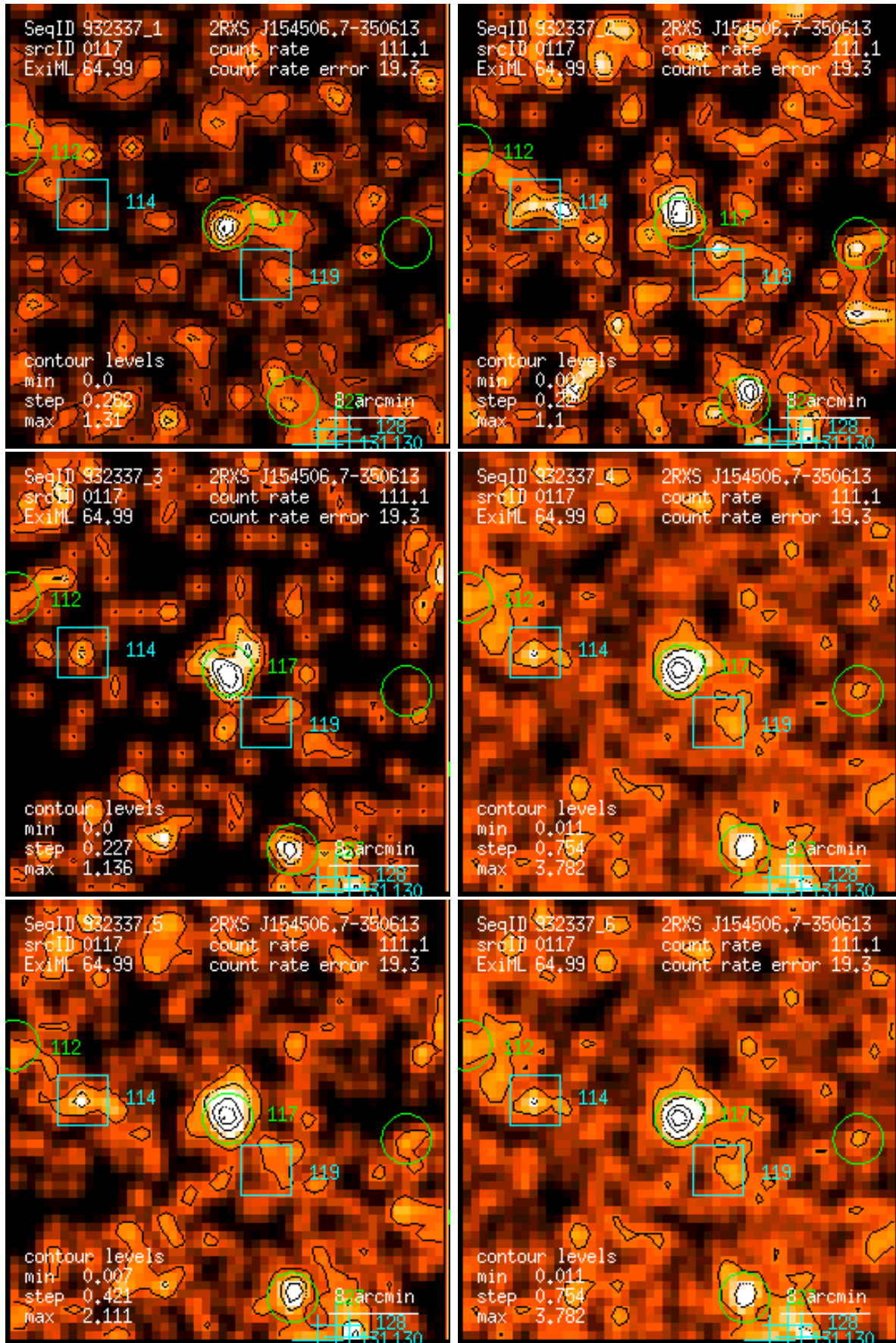
Figure 117: RASS 932337: detection 0117: band rate images, Gaussian filter: (1) PSPC channels 11 – 41, (2) 52 – 90, (3) 91 – 201, (4) 11 – 235, (5) 52 – 201, (6) 11 – 201. Broad band rates in counts/ks. Band rate contour levels in counts/ks/arcmin 2 .
