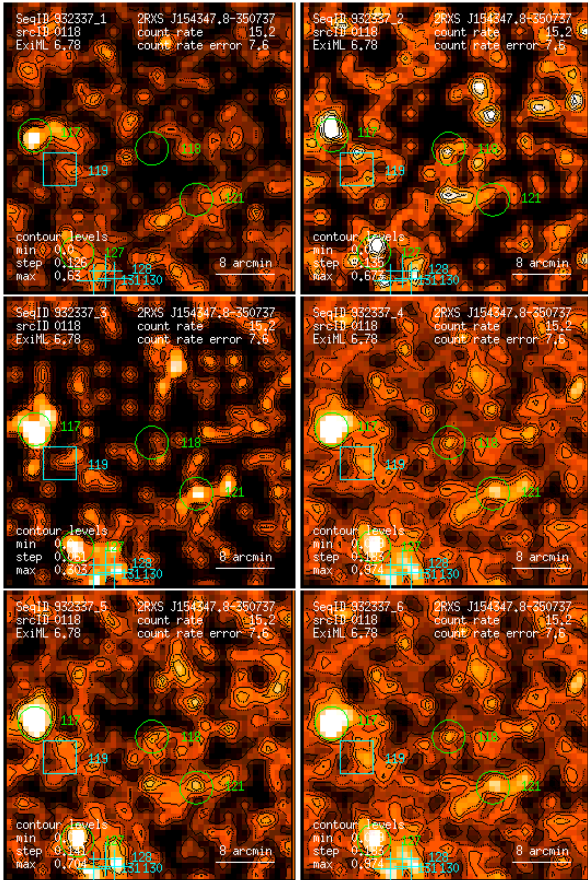
Figure 118: RASS 932337: detection 0118: band rate images, Gaussian filter: (1) PSPC channels 11 – 41, (2) 52 – 90, (3) 91 – 201, (4) 11 – 235, (5) 52 – 201, (6) 11 – 201. Broad band rates in counts/ks. Band rate contour levels in counts/ks/arcmin 2 .
