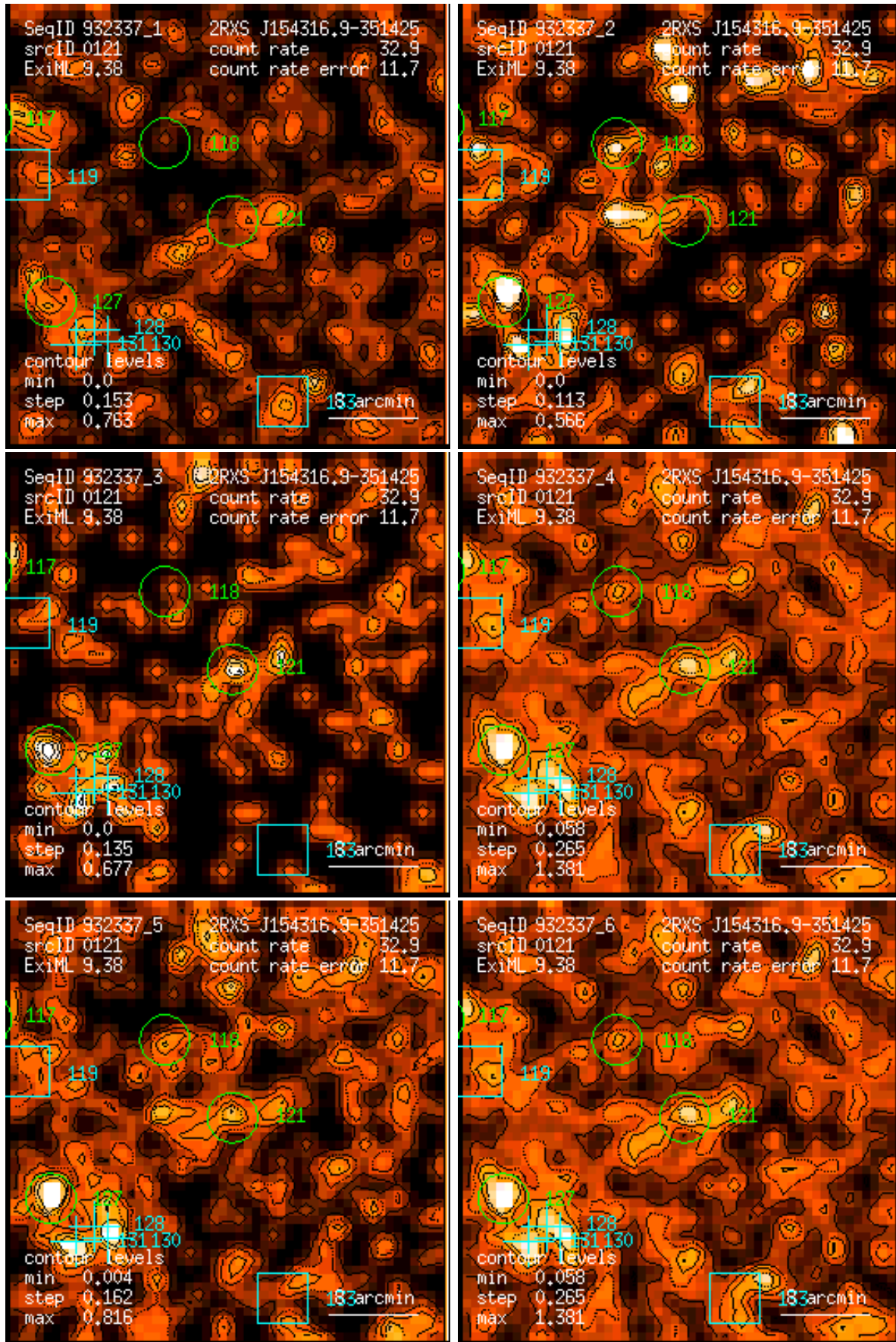
Figure 121: RASS 932337: detection 0121: band rate images, Gaussian filter: (1) PSPC channels 11 – 41, (2) 52 – 90, (3) 91 – 201, (4) 11 – 235, (5) 52 – 201, (6) 11 – 201. Broad band rates in counts/ks. Band rate contour levels in counts/ks/arcmin 2 .
