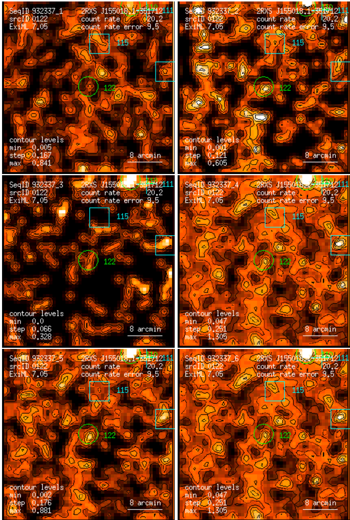
Figure 122: RASS 932337: detection 0122: band rate images, Gaussian filter: (1) PSPC channels 11 – 41, (2) 52 – 90, (3) 91 – 201, (4) 11 – 235, (5) 52 – 201, (6) 11 – 201. Broad band rates in counts/ks. Band rate contour levels in counts/ks/arcmin 2 .
