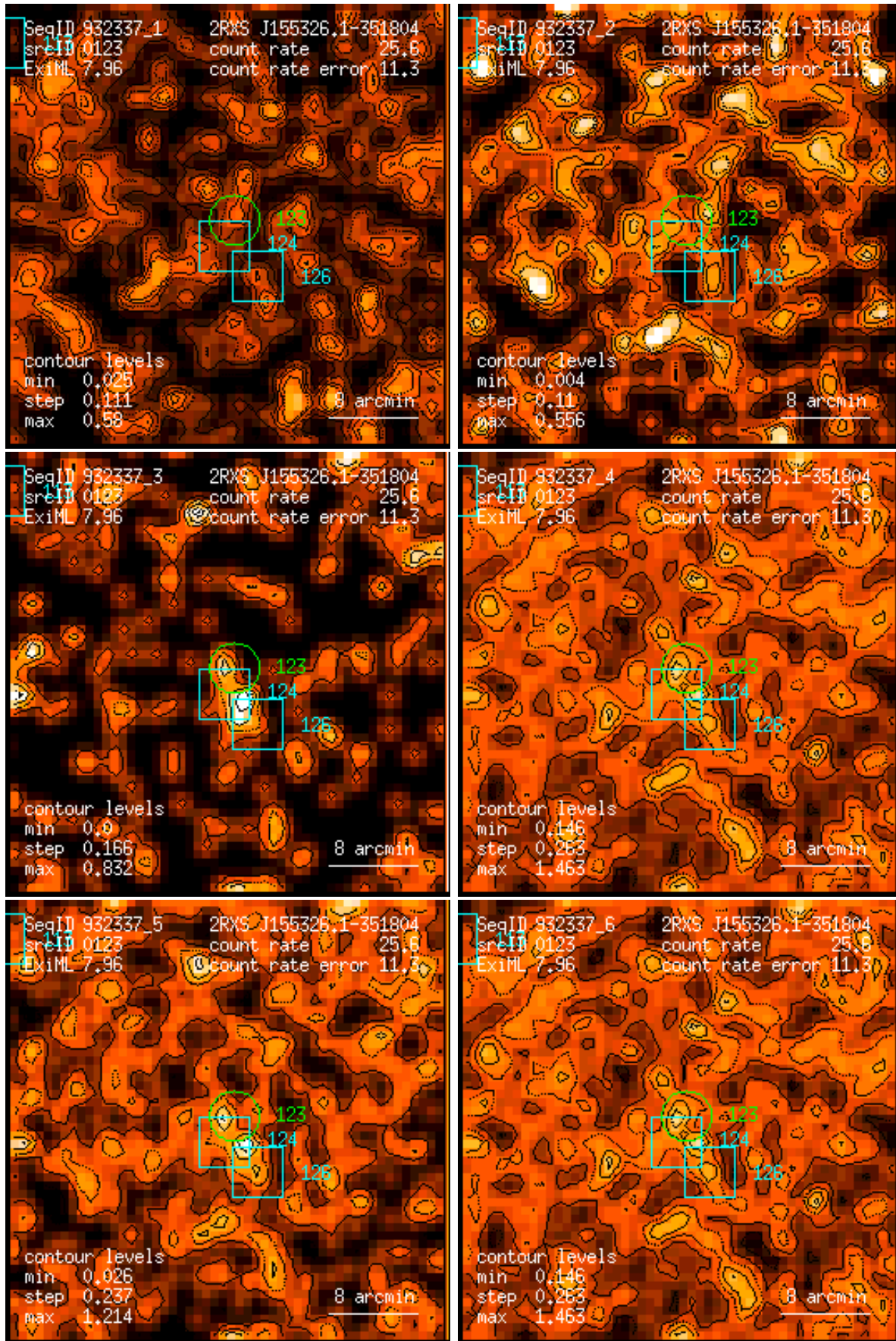
Figure 123: RASS 932337: detection 0123: band rate images, Gaussian filter: (1) PSPC channels 11 – 41, (2) 52 – 90, (3) 91 – 201, (4) 11 – 235, (5) 52 – 201, (6) 11 – 201. Broad band rates in counts/ks. Band rate contour levels in counts/ks/arcmin 2 .
